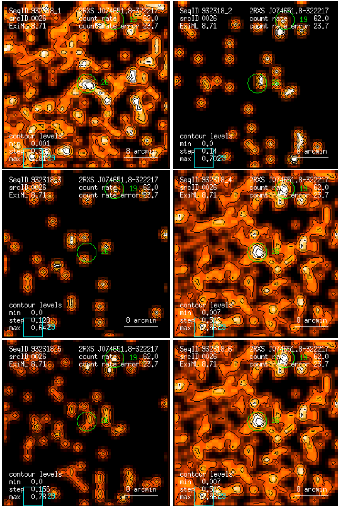
Figure 26: RASS 932318: detection 0026: band rate images, Gaussian filter: (1) PSPC channels 11 – 41, (2) 52 – 90, (3) 91 – 201, (4) 11 – 235, (5) 52 – 201, (6) 11 – 201. Broad band rates in counts/ks. Band rate contour levels in counts/ks/arcmin 2 .
