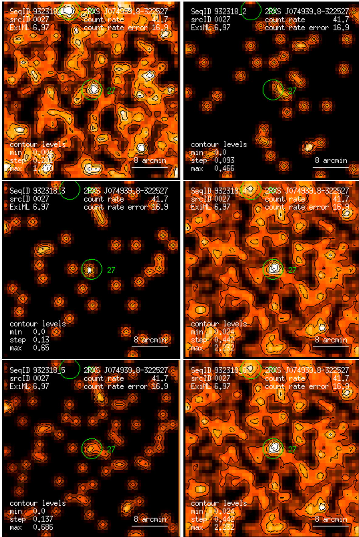
Figure 27: RASS 932318: detection 0027: band rate images, Gaussian filter: (1) PSPC channels 11 – 41, (2) 52 – 90, (3) 91 – 201, (4) 11 – 235, (5) 52 – 201, (6) 11 – 201. Broad band rates in counts/ks. Band rate contour levels in counts/ks/arcmin 2 .
