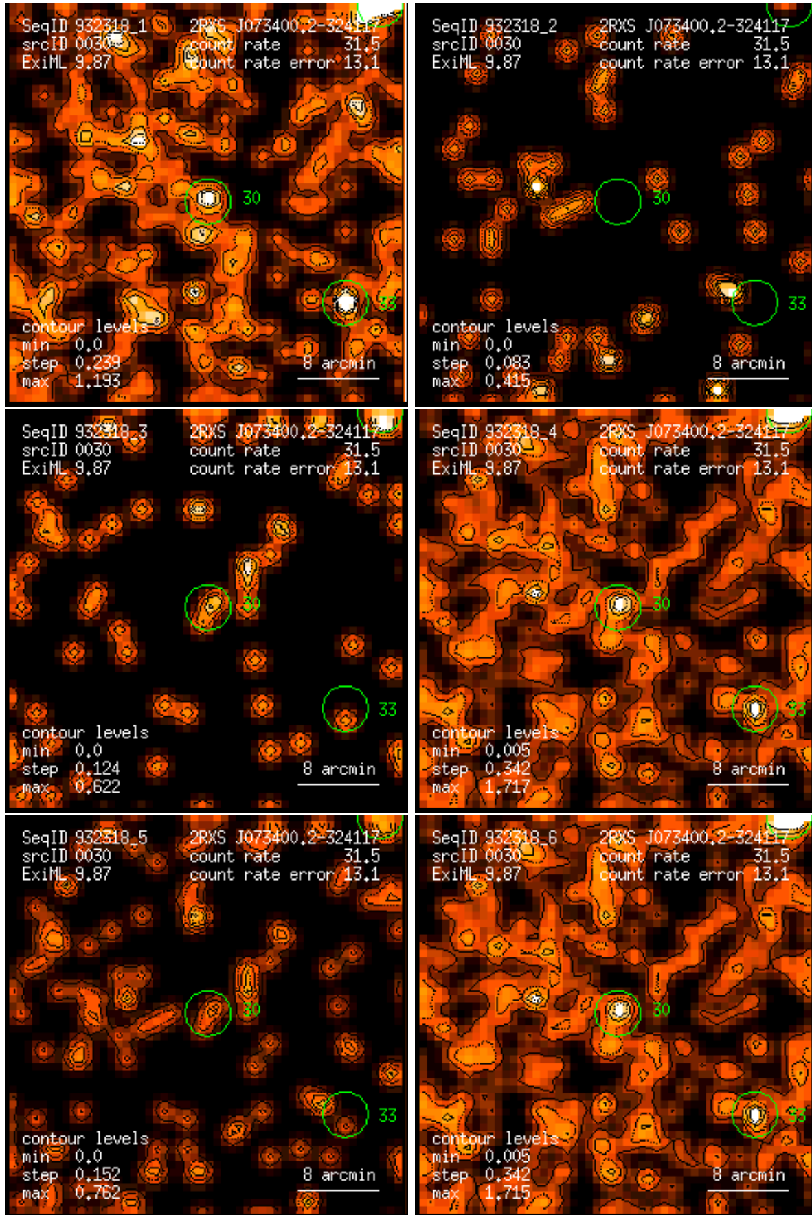
Figure 30: RASS 932318: detection 0030: band rate images, Gaussian filter: (1) PSPC channels 11 – 41, (2) 52 – 90, (3) 91 – 201, (4) 11 – 235, (5) 52 – 201, (6) 11 – 201. Broad band rates in counts/ks. Band rate contour levels in counts/ks/arcmin 2 .
