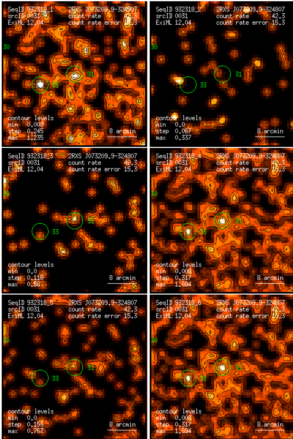
Figure 31: RASS 932318: detection 0031: band rate images, Gaussian filter: (1) PSPC channels 11 – 41, (2) 52 – 90, (3) 91 – 201, (4) 11 – 235, (5) 52 – 201, (6) 11 – 201. Broad band rates in counts/ks. Band rate contour levels in counts/ks/arcmin 2 .
