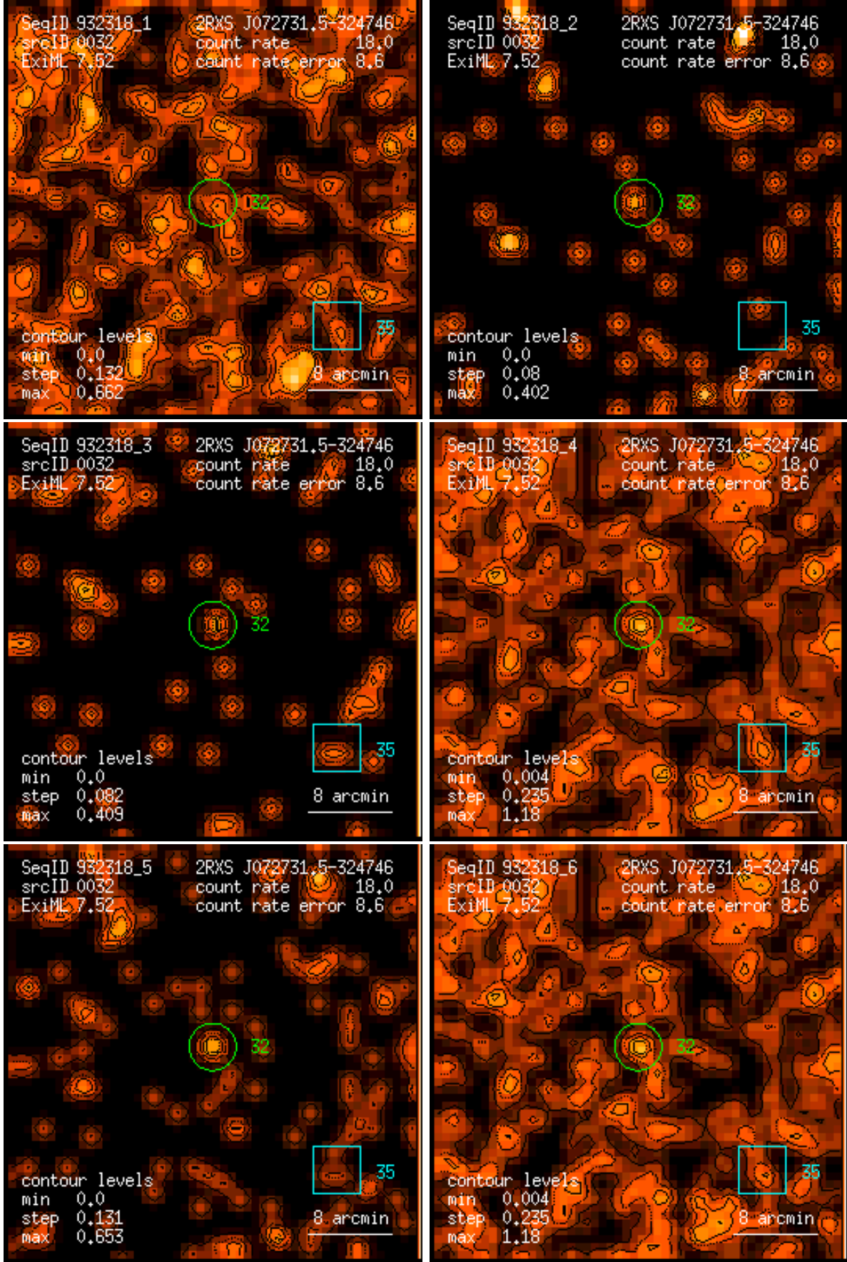
Figure 32: RASS 932318: detection 0032: band rate images, Gaussian filter: (1) PSPC channels 11 – 41, (2) 52 – 90, (3) 91 – 201, (4) 11 – 235, (5) 52 – 201, (6) 11 – 201. Broad band rates in counts/ks. Band rate contour levels in counts/ks/arcmin 2 .
