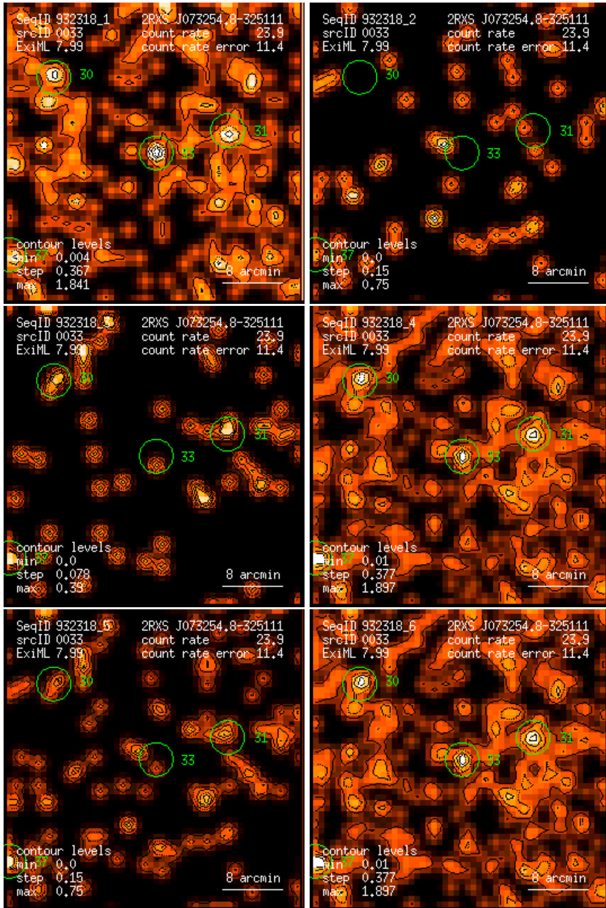
Figure 33: RASS 932318: detection 0033: band rate images, Gaussian filter: (1) PSPC channels 11 – 41, (2) 52 – 90, (3) 91 – 201, (4) 11 – 235, (5) 52 – 201, (6) 11 – 201. Broad band rates in counts/ks. Band rate contour levels in counts/ks/arcmin 2 .
