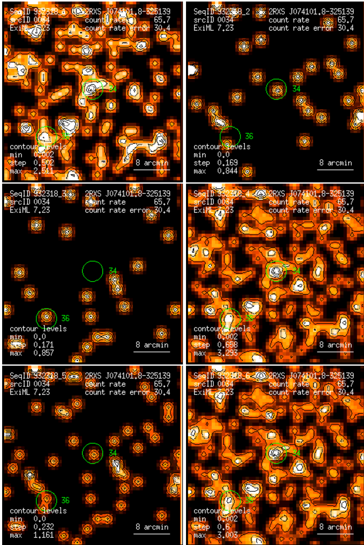
Figure 34: RASS 932318: detection 0034: band rate images, Gaussian filter: (1) PSPC channels 11 – 41, (2) 52 – 90, (3) 91 – 201, (4) 11 – 235, (5) 52 – 201, (6) 11 – 201. Broad band rates in counts/ks. Band rate contour levels in counts/ks/arcmin 2 .
