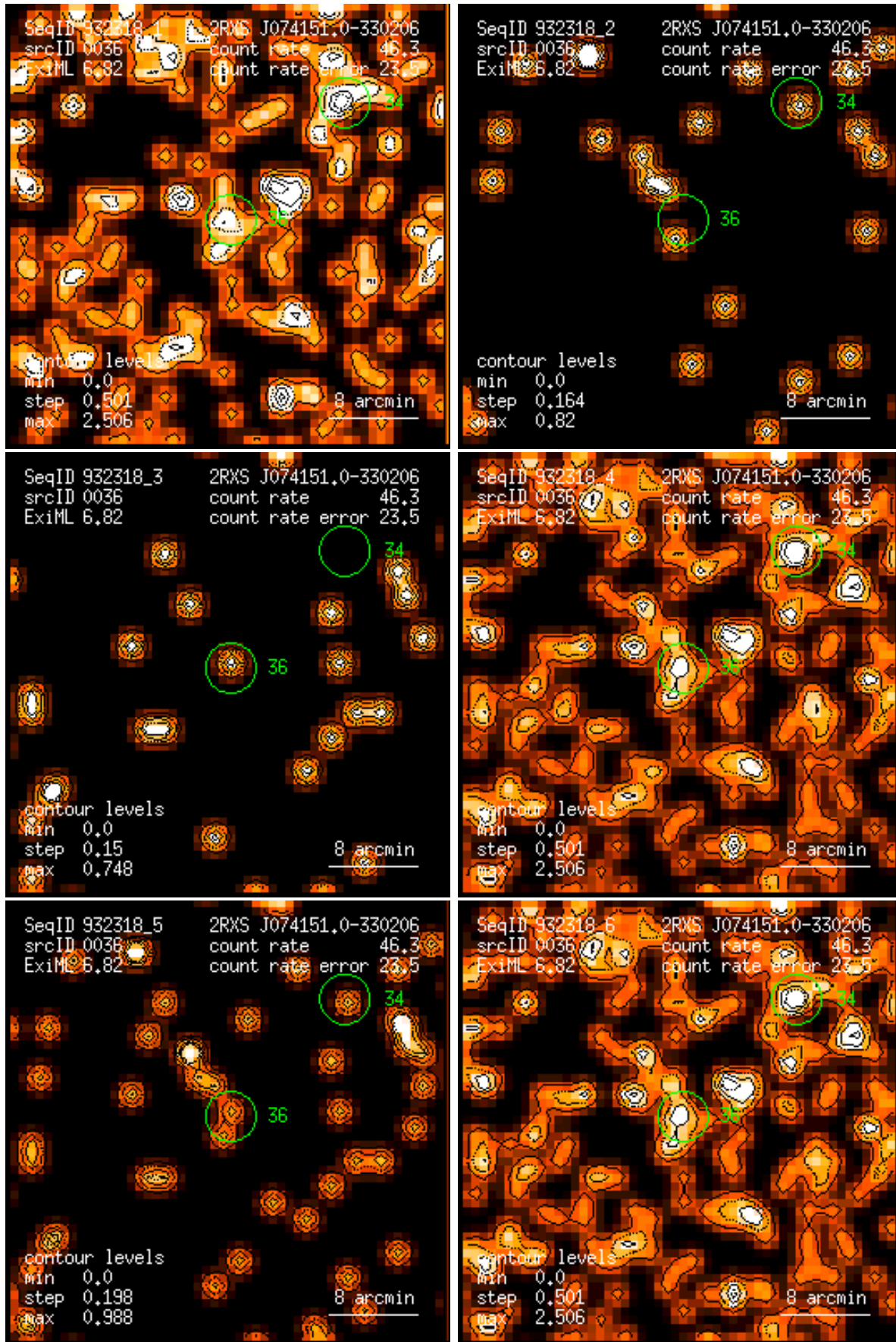
Figure 36: RASS 932318: detection 0036: band rate images, Gaussian filter: (1) PSPC channels 11 – 41, (2) 52 – 90, (3) 91 – 201, (4) 11 – 235, (5) 52 – 201, (6) 11 – 201. Broad band rates in counts/ks. Band rate contour levels in counts/ks/arcmin 2 .
