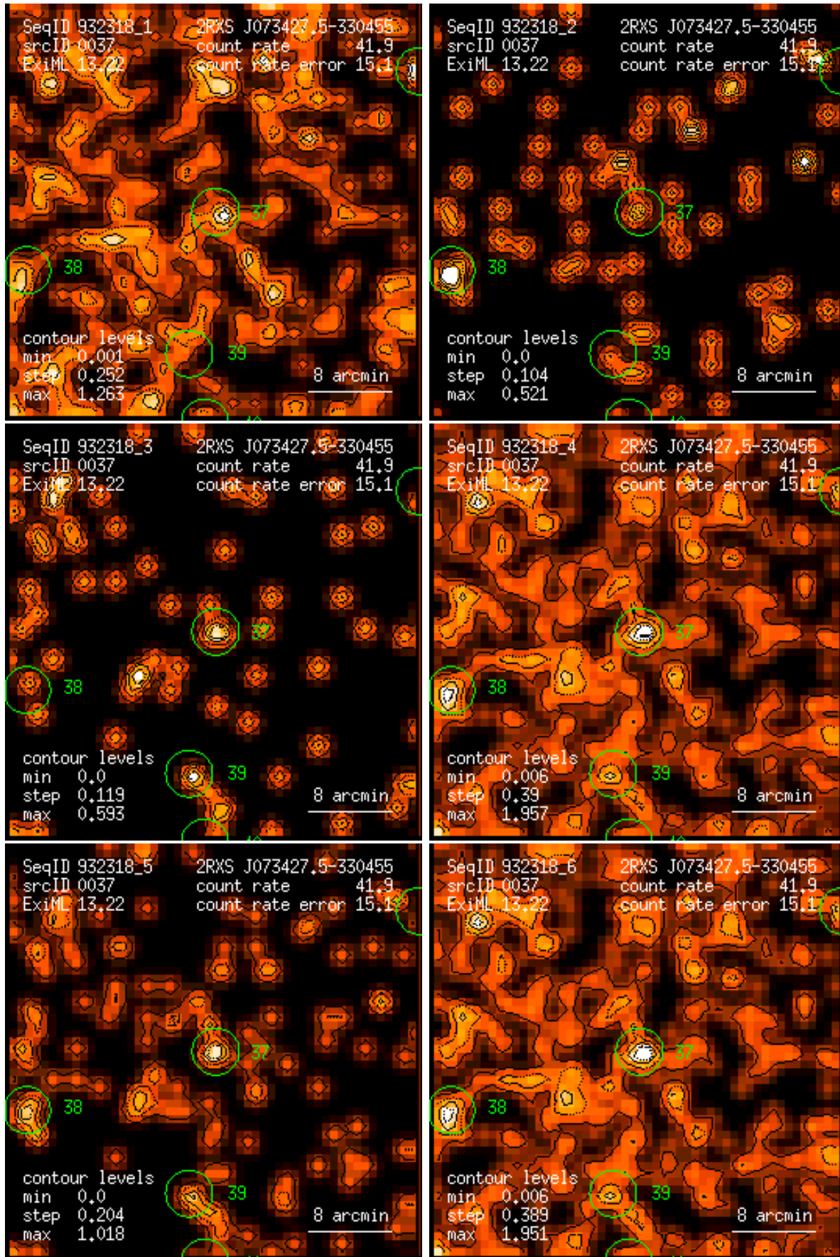
Figure 37: RASS 932318: detection 0037: band rate images, Gaussian filter: (1) PSPC channels 11 – 41, (2) 52 – 90, (3) 91 – 201, (4) 11 – 235, (5) 52 – 201, (6) 11 – 201. Broad band rates in counts/ks. Band rate contour levels in counts/ks/arcmin 2 .
