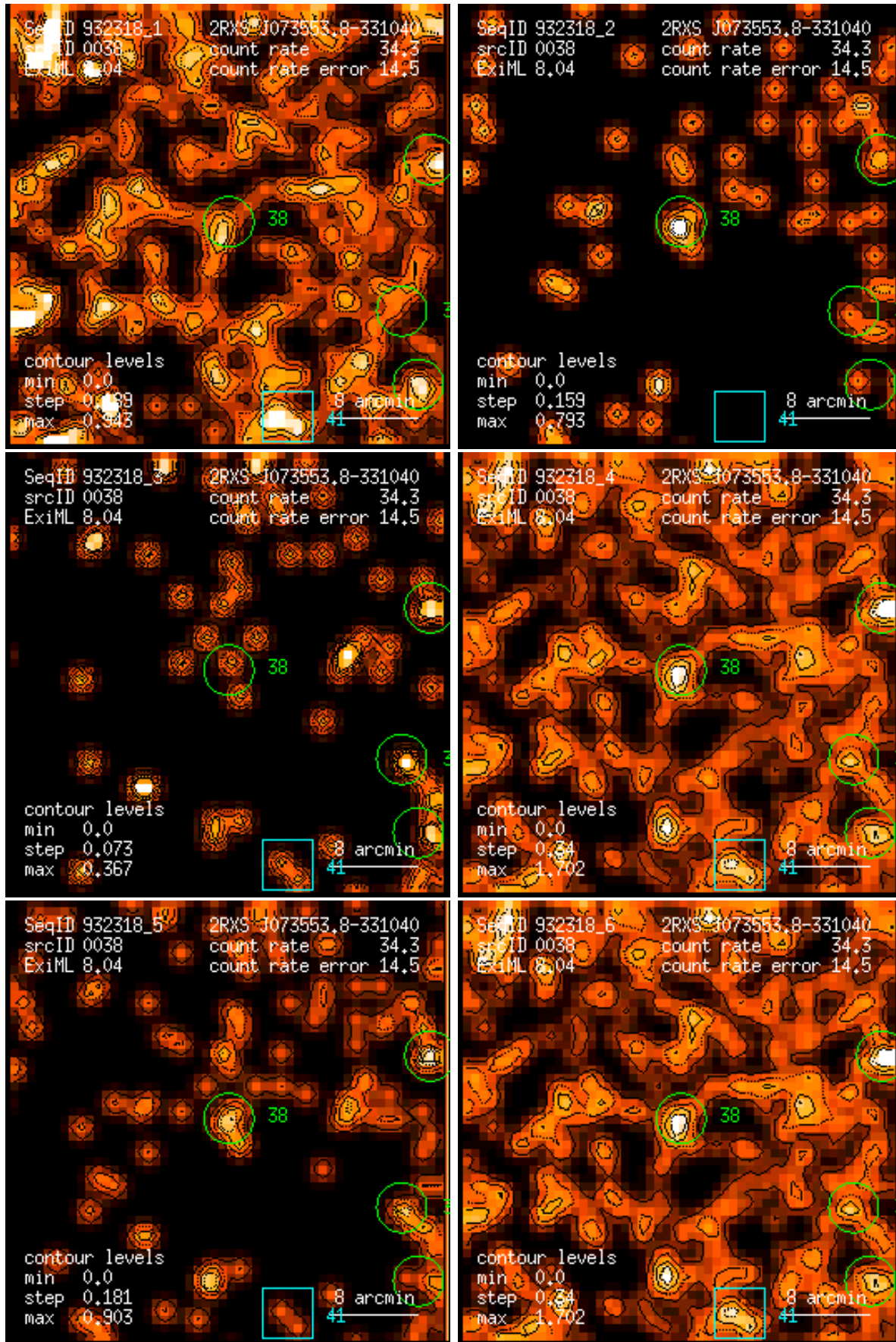
Figure 38: RASS 932318: detection 0038: band rate images, Gaussian filter: (1) PSPC channels 11 – 41, (2) 52 – 90, (3) 91 – 201, (4) 11 – 235, (5) 52 – 201, (6) 11 – 201. Broad band rates in counts/ks. Band rate contour levels in counts/ks/arcmin 2 .
