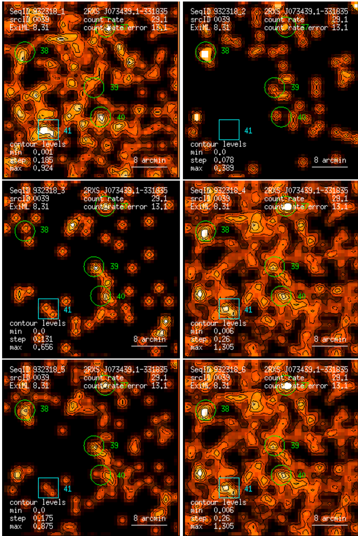
Figure 39: RASS 932318: detection 0039: band rate images, Gaussian filter: (1) PSPC channels 11 – 41, (2) 52 – 90, (3) 91 – 201, (4) 11 – 235, (5) 52 – 201, (6) 11 – 201. Broad band rates in counts/ks. Band rate contour levels in counts/ks/arcmin 2 .
