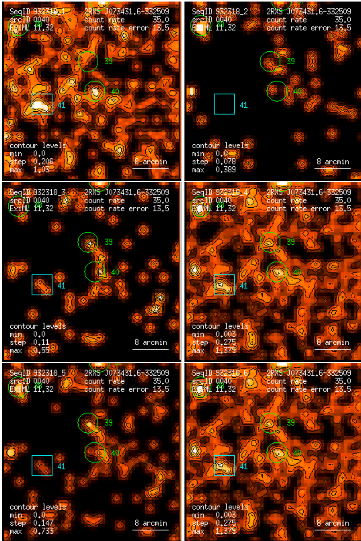
Figure 40: RASS 932318: detection 0040: band rate images, Gaussian filter: (1) PSPC channels 11 – 41, (2) 52 – 90, (3) 91 – 201, (4) 11 – 235, (5) 52 – 201, (6) 11 – 201. Broad band rates in counts/ks. Band rate contour levels in counts/ks/arcmin 2 .
