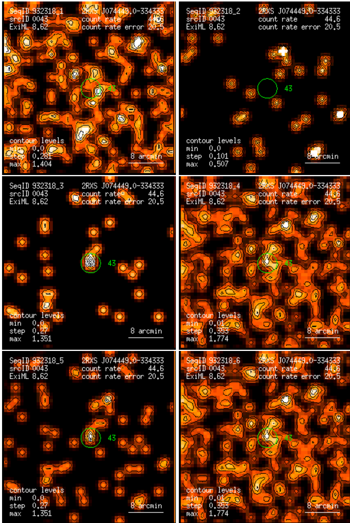
Figure 43: RASS 932318: detection 0043: band rate images, Gaussian filter: (1) PSPC channels 11 – 41, (2) 52 – 90, (3) 91 – 201, (4) 11 – 235, (5) 52 – 201, (6) 11 – 201. Broad band rates in counts/ks. Band rate contour levels in counts/ks/arcmin 2 .
