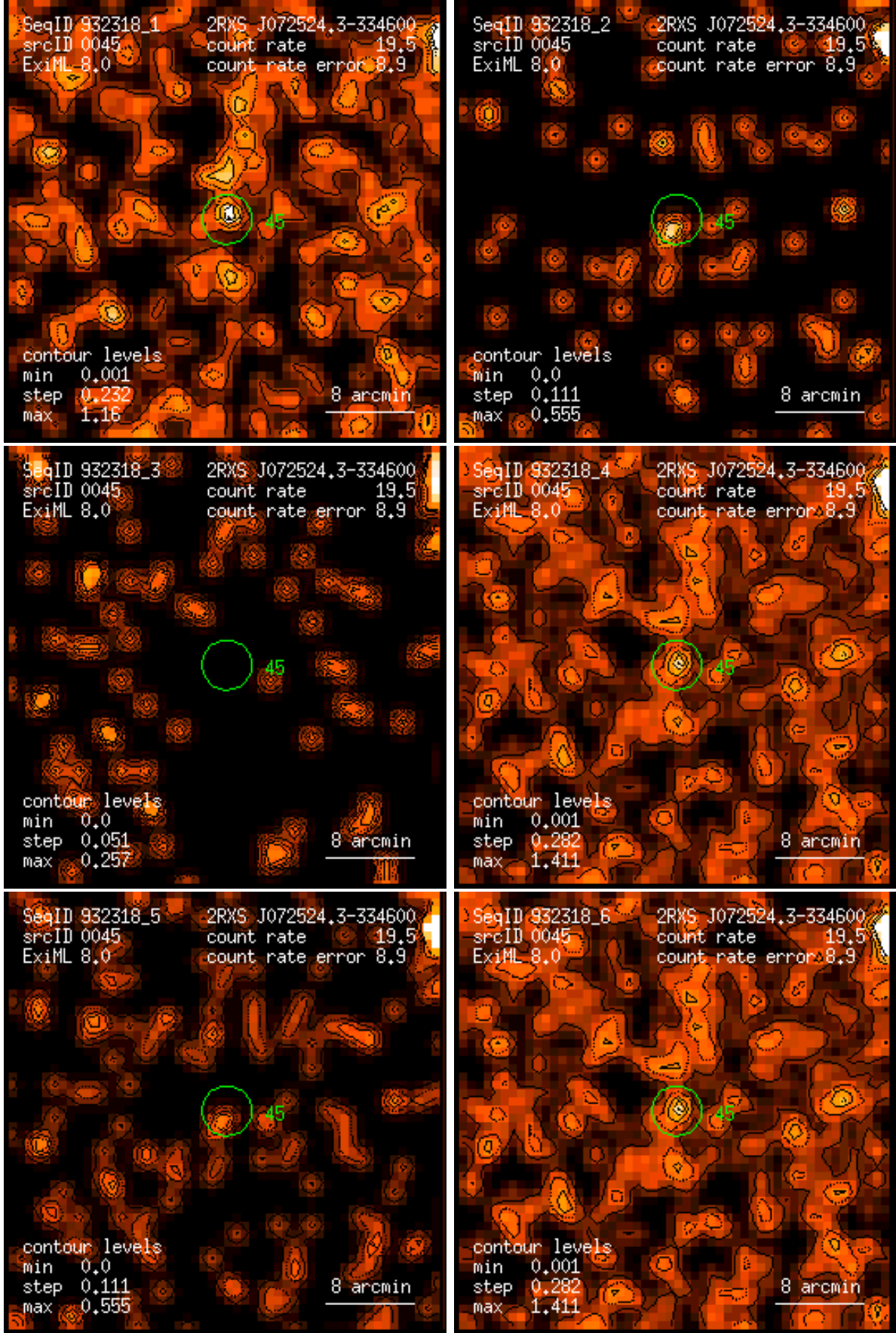
Figure 45: RASS 932318: detection 0045: band rate images, Gaussian filter: (1) PSPC channels 11 – 41, (2) 52 – 90, (3) 91 – 201, (4) 11 – 235, (5) 52 – 201, (6) 11 – 201. Broad band rates in counts/ks. Band rate contour levels in counts/ks/arcmin 2 .
