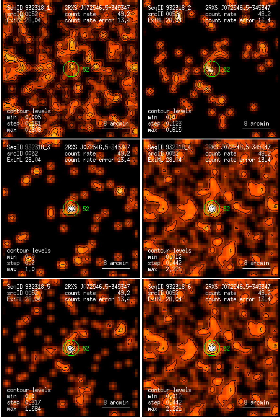
Figure 52: RASS 932318: detection 0052: band rate images, Gaussian filter: (1) PSPC channels 11 – 41, (2) 52 – 90, (3) 91 – 201, (4) 11 – 235, (5) 52 – 201, (6) 11 – 201. Broad band rates in counts/ks. Band rate contour levels in counts/ks/arcmin 2 .
