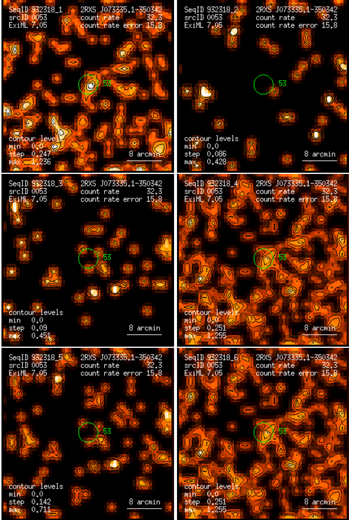
Figure 53: RASS 932318: detection 0053: band rate images, Gaussian filter: (1) PSPC channels 11 – 41, (2) 52 – 90, (3) 91 – 201, (4) 11 – 235, (5) 52 – 201, (6) 11 – 201. Broad band rates in counts/ks. Band rate contour levels in counts/ks/arcmin 2 .
