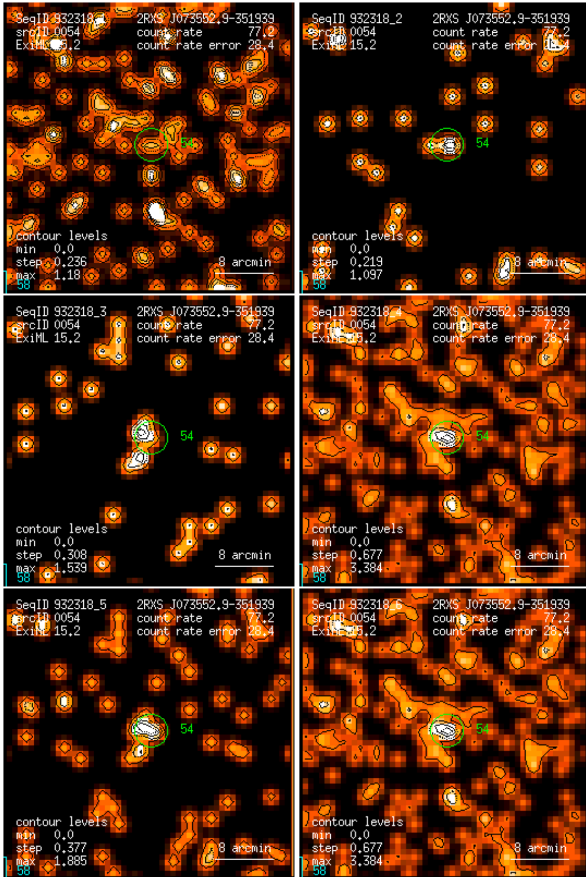
Figure 54: RASS 932318: detection 0054: band rate images, Gaussian filter: (1) PSPC channels 11 – 41, (2) 52 – 90, (3) 91 – 201, (4) 11 – 235, (5) 52 – 201, (6) 11 – 201. Broad band rates in counts/ks. Band rate contour levels in counts/ks/arcmin 2 .
