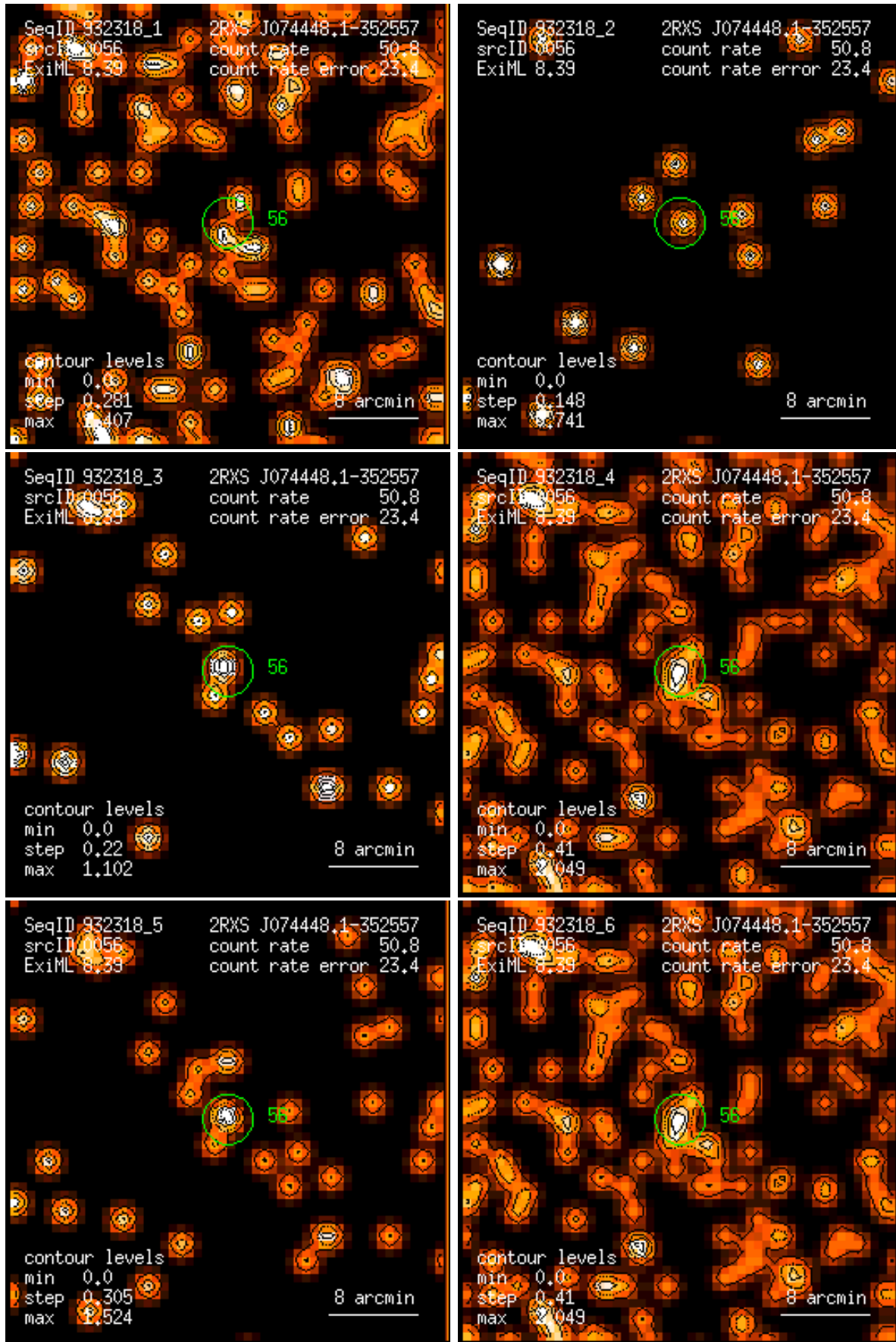
Figure 56: RASS 932318: detection 0056: band rate images, Gaussian filter: (1) PSPC channels 11 – 41, (2) 52 – 90, (3) 91 – 201, (4) 11 – 235, (5) 52 – 201, (6) 11 – 201. Broad band rates in counts/ks. Band rate contour levels in counts/ks/arcmin 2 .
