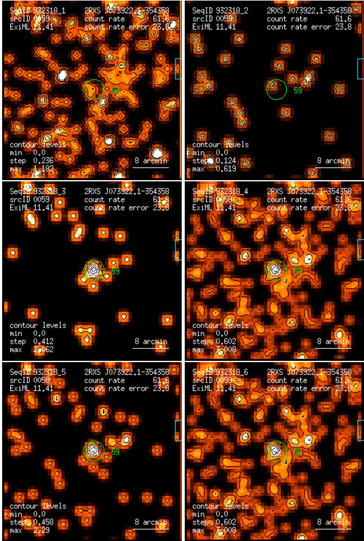
Figure 59: RASS 932318: detection 0059: band rate images, Gaussian filter: (1) PSPC channels 11 – 41, (2) 52 – 90, (3) 91 – 201, (4) 11 – 235, (5) 52 – 201, (6) 11 – 201. Broad band rates in counts/ks. Band rate contour levels in counts/ks/arcmin 2 .
