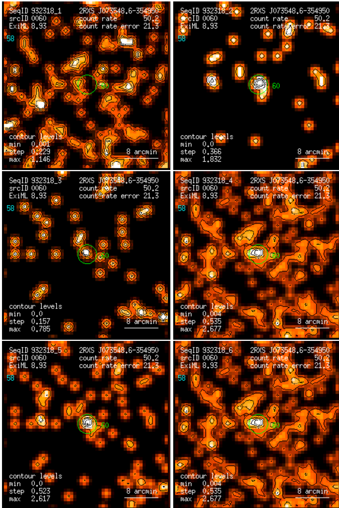
Figure 60: RASS 932318: detection 0060: band rate images, Gaussian filter: (1) PSPC channels 11 – 41, (2) 52 – 90, (3) 91 – 201, (4) 11 – 235, (5) 52 – 201, (6) 11 – 201. Broad band rates in counts/ks. Band rate contour levels in counts/ks/arcmin 2 .
