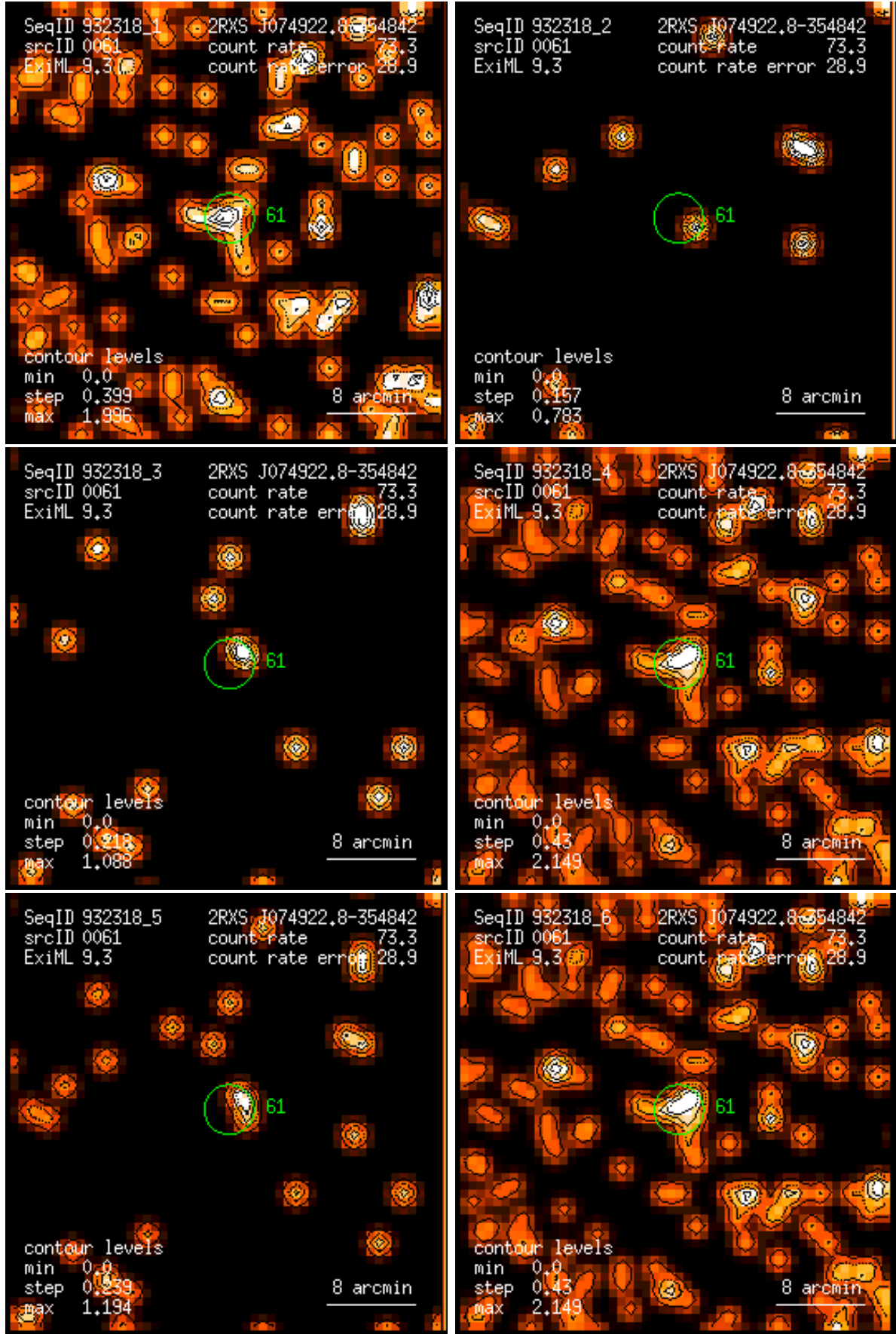
Figure 61: RASS 932318: detection 0061: band rate images, Gaussian filter: (1) PSPC channels 11 – 41, (2) 52 – 90, (3) 91 – 201, (4) 11 – 235, (5) 52 – 201, (6) 11 – 201. Broad band rates in counts/ks. Band rate contour levels in counts/ks/arcmin 2 .
