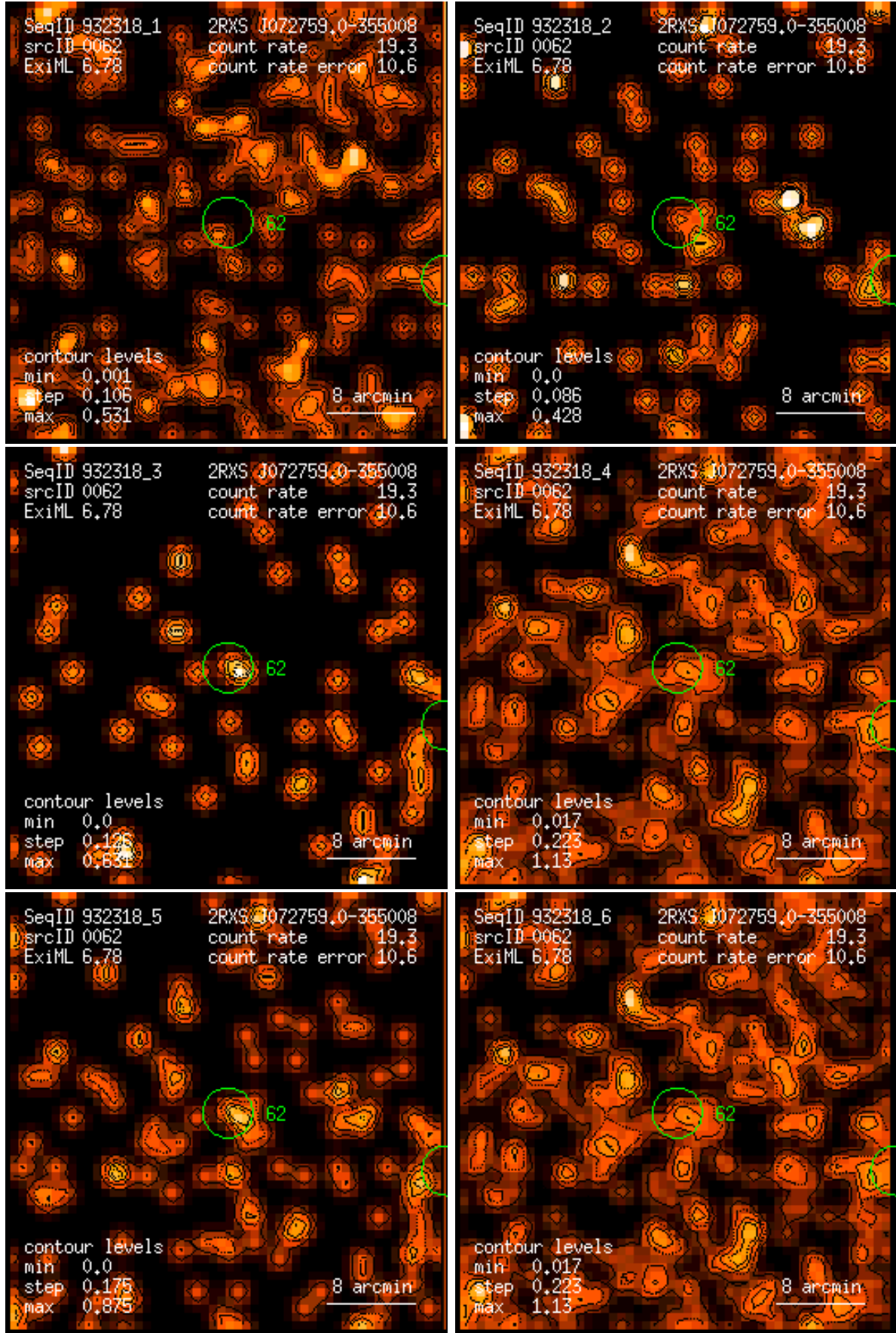
Figure 62: RASS 932318: detection 0062: band rate images, Gaussian filter: (1) PSPC channels 11 – 41, (2) 52 – 90, (3) 91 – 201, (4) 11 – 235, (5) 52 – 201, (6) 11 – 201. Broad band rates in counts/ks. Band rate contour levels in counts/ks/arcmin 2 .
