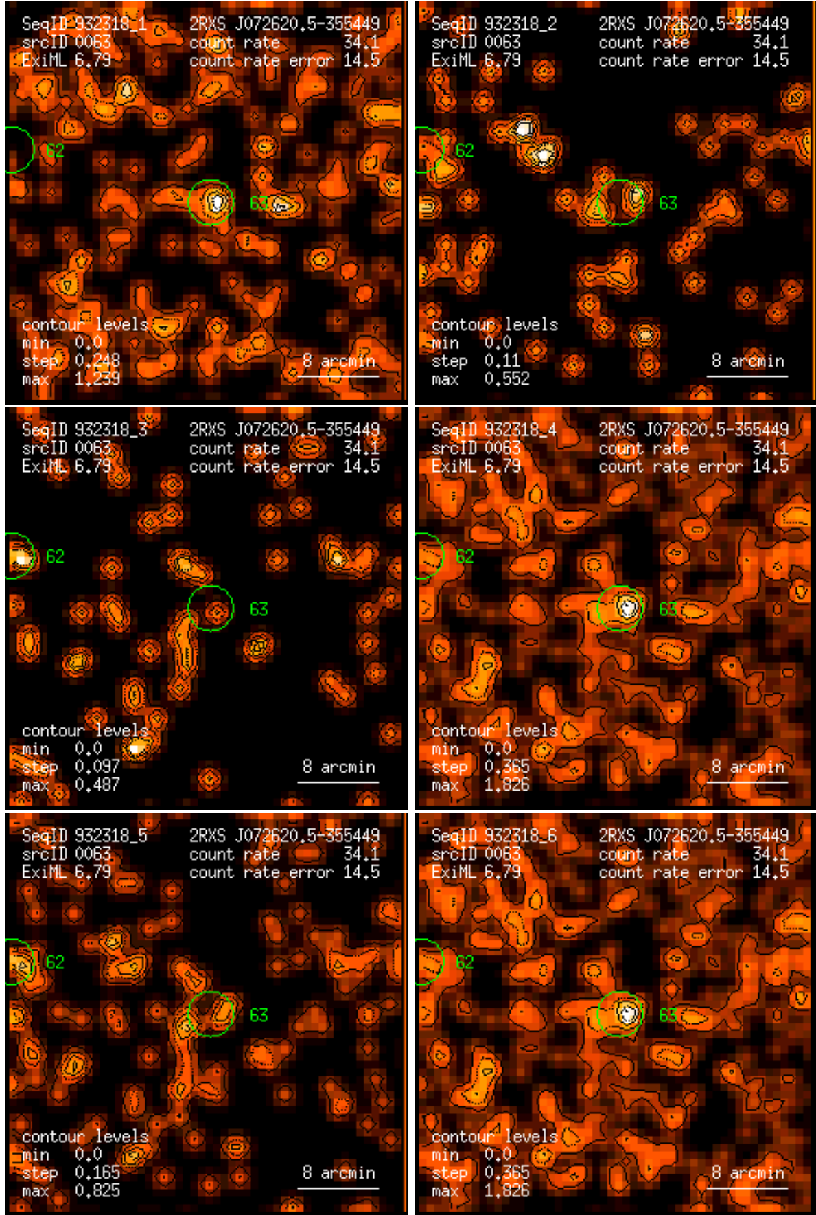
Figure 63: RASS 932318: detection 0063: band rate images, Gaussian filter: (1) PSPC channels 11 – 41, (2) 52 – 90, (3) 91 – 201, (4) 11 – 235, (5) 52 – 201, (6) 11 – 201. Broad band rates in counts/ks. Band rate contour levels in counts/ks/arcmin 2 .
