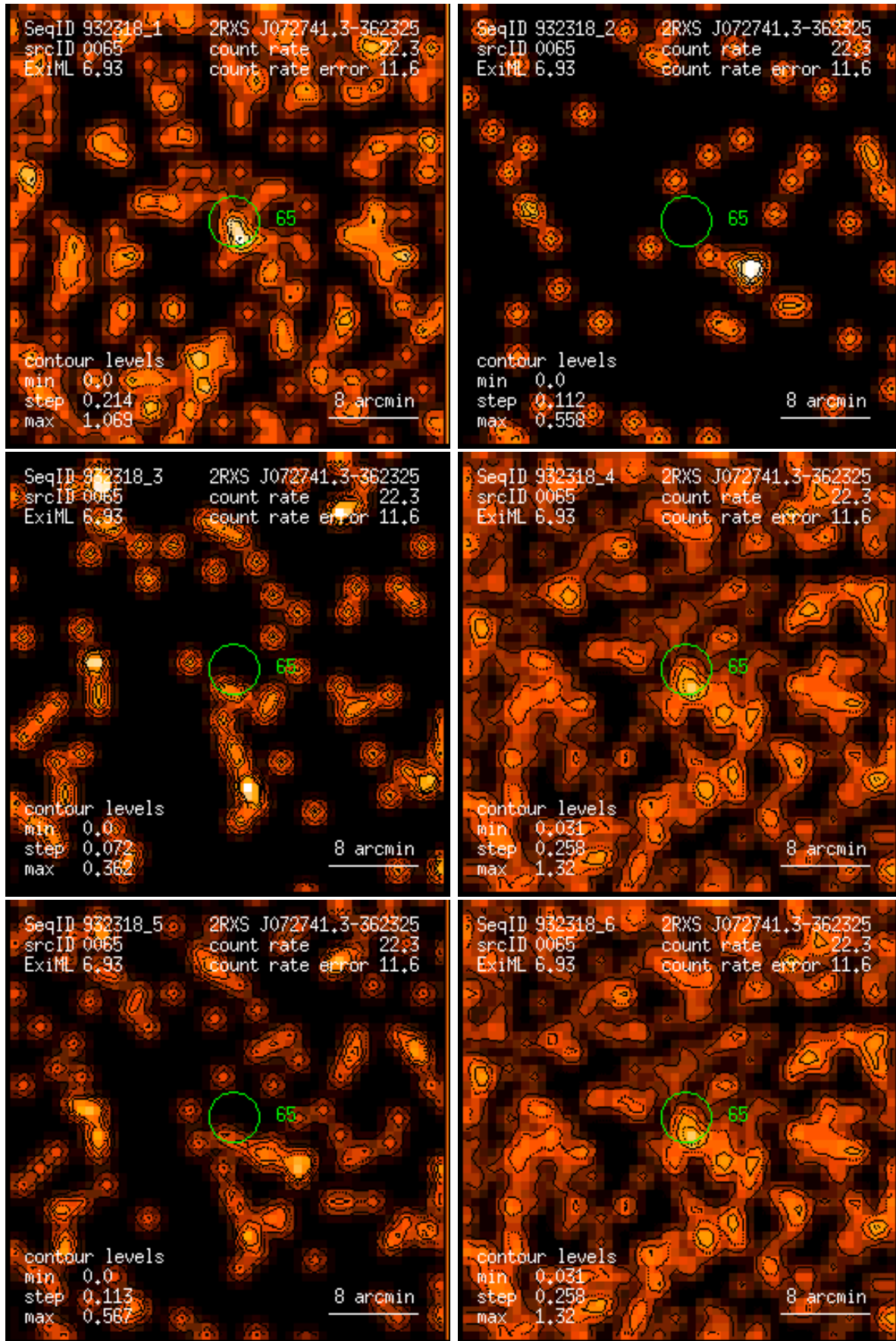
Figure 65: RASS 932318: detection 0065: band rate images, Gaussian filter: (1) PSPC channels 11 – 41, (2) 52 – 90, (3) 91 – 201, (4) 11 – 235, (5) 52 – 201, (6) 11 – 201. Broad band rates in counts/ks. Band rate contour levels in counts/ks/arcmin 2 .
