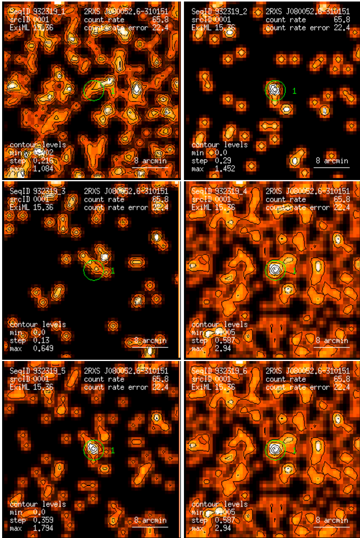
Figure 1: RASS 932319: detection 0001: band rate images, Gaussian filter: (1) PSPC channels 11 – 41, (2) 52 – 90, (3) 91 – 201, (4) 11 – 235, (5) 52 – 201, (6) 11 – 201. Broad band rates in counts/ks. Band rate contour levels in counts/ks/arcmin 2 .
