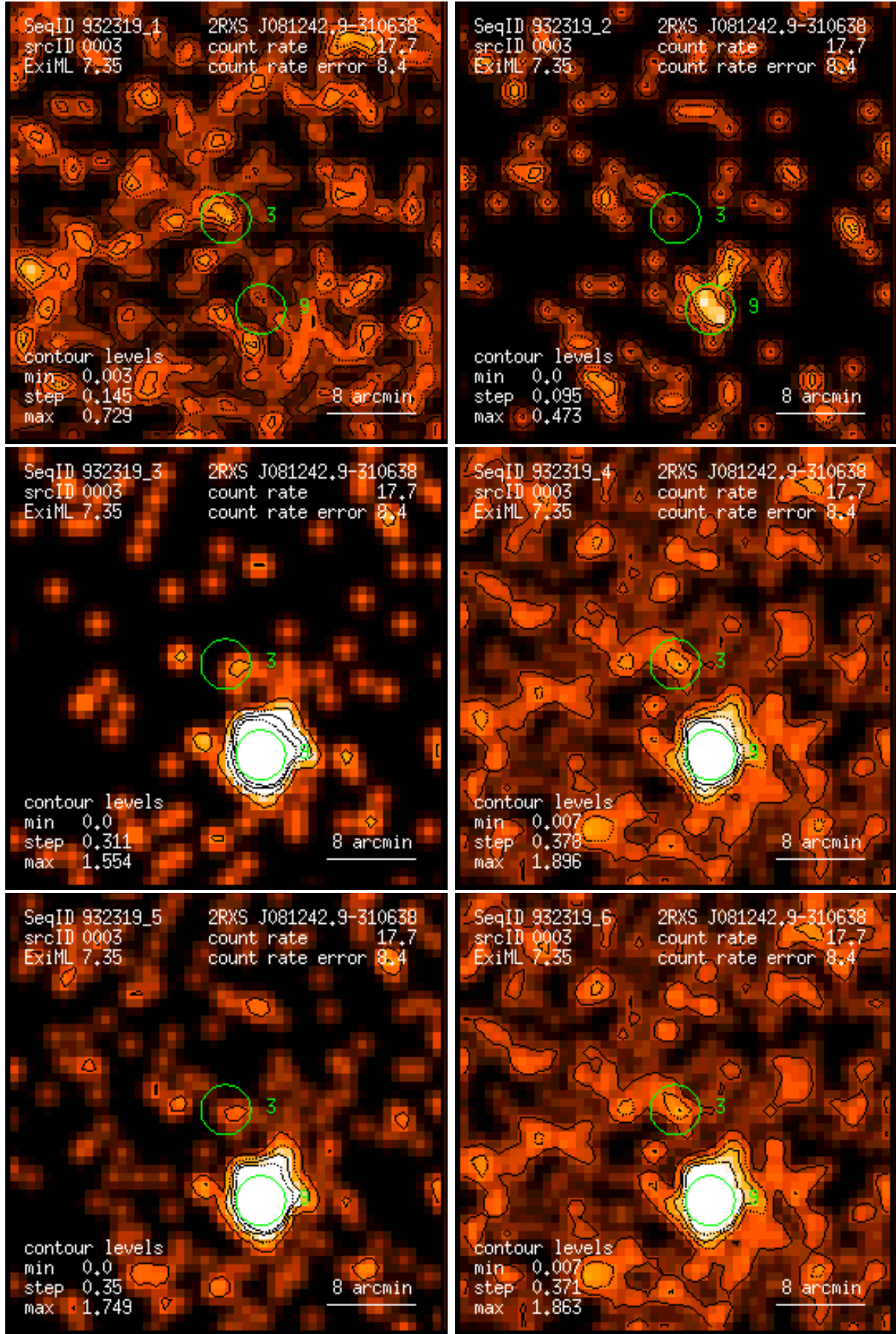
Figure 3: RASS 932319: detection 0003: band rate images, Gaussian filter: (1) PSPC channels 11 – 41, (2) 52 – 90, (3) 91 – 201, (4) 11 – 235, (5) 52 – 201, (6) 11 – 201. Broad band rates in counts/ks. Band rate contour levels in counts/ks/arcmin 2 .
