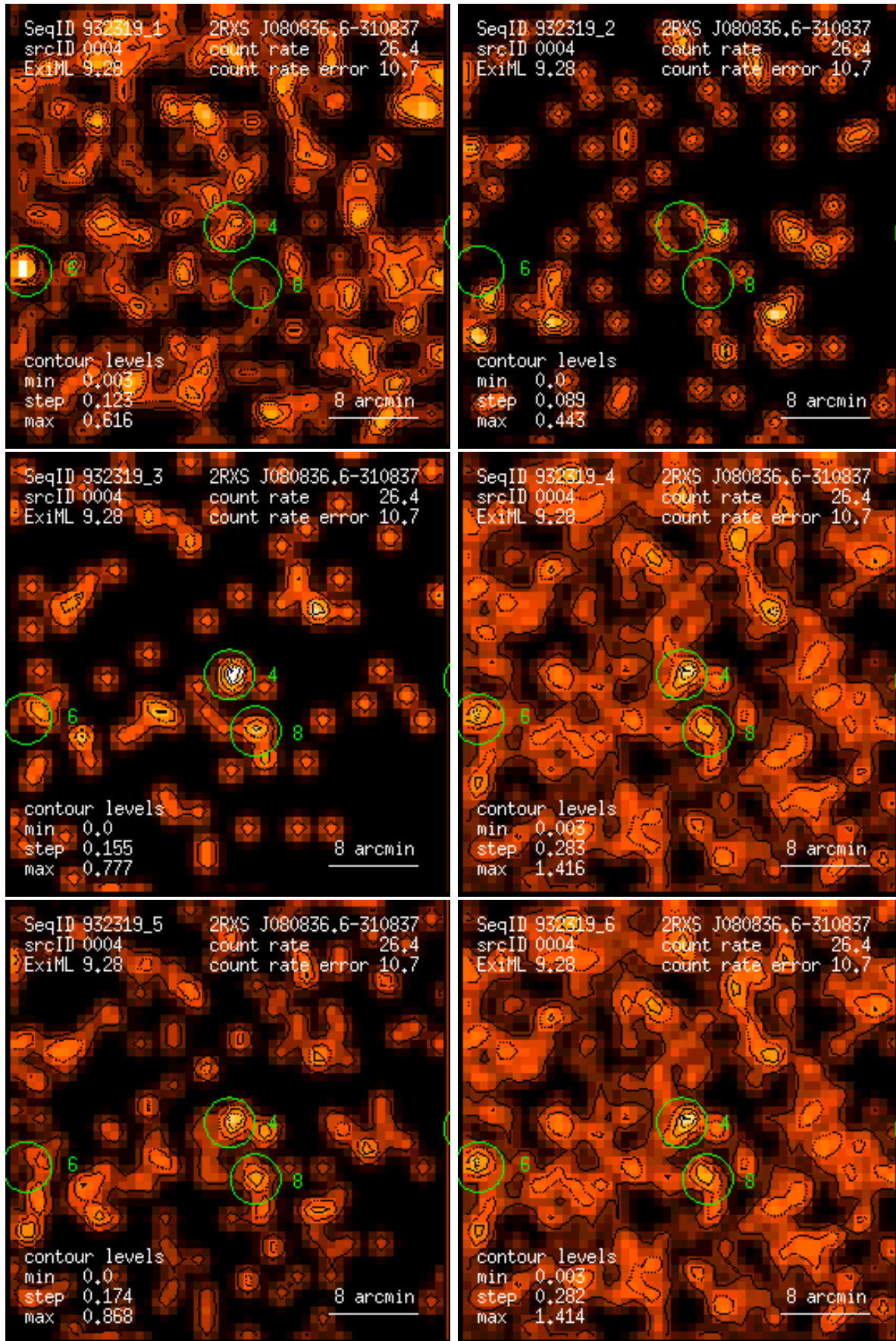
Figure 4: RASS 932319: detection 0004: band rate images, Gaussian filter: (1) PSPC channels 11 – 41, (2) 52 – 90, (3) 91 – 201, (4) 11 – 235, (5) 52 – 201, (6) 11 – 201. Broad band rates in counts/ks. Band rate contour levels in counts/ks/arcmin 2 .
