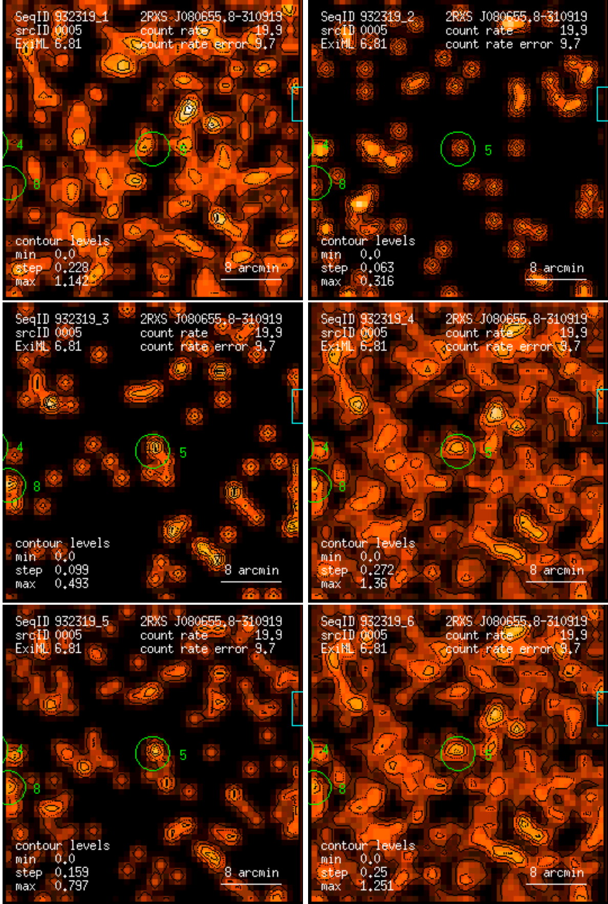
Figure 5: RASS 932319: detection 0005: band rate images, Gaussian filter: (1) PSPC channels 11 – 41, (2) 52 – 90, (3) 91 – 201, (4) 11 – 235, (5) 52 – 201, (6) 11 – 201. Broad band rates in counts/ks. Band rate contour levels in counts/ks/arcmin 2 .
