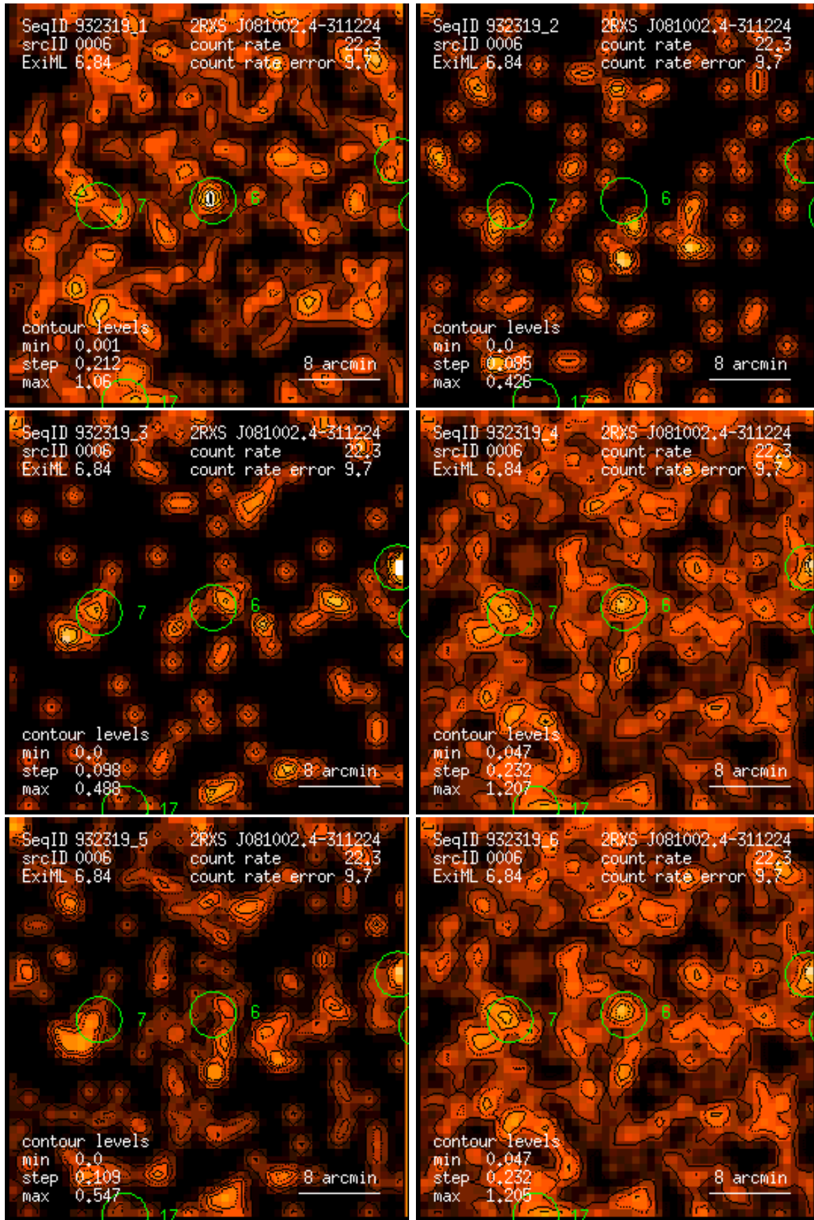
Figure 6: RASS 932319: detection 0006: band rate images, Gaussian filter: (1) PSPC channels 11 – 41, (2) 52 – 90, (3) 91 – 201, (4) 11 – 235, (5) 52 – 201, (6) 11 – 201. Broad band rates in counts/ks. Band rate contour levels in counts/ks/arcmin 2 .
