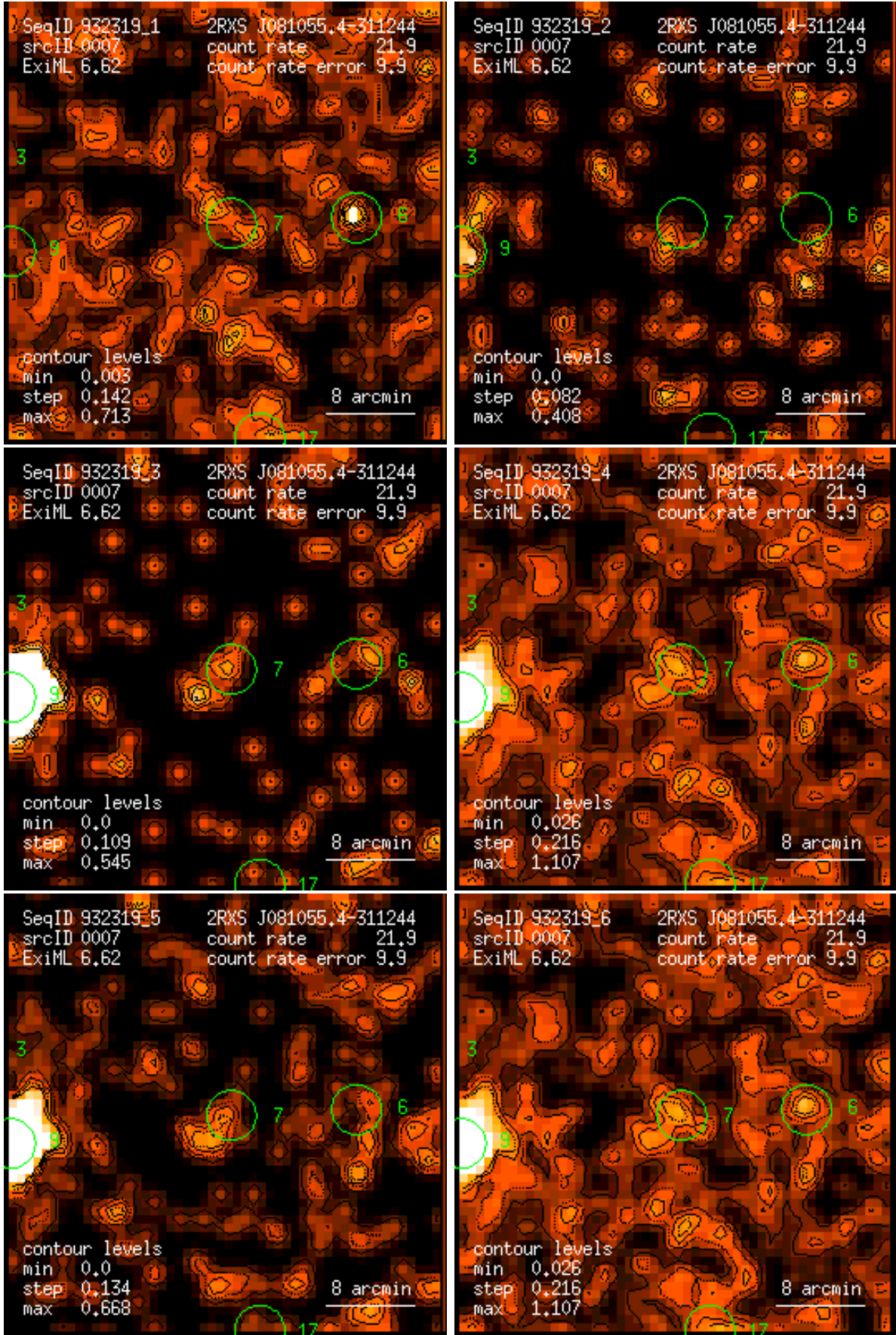
Figure 7: RASS 932319: detection 0007: band rate images, Gaussian filter: (1) PSPC channels 11 – 41, (2) 52 – 90, (3) 91 – 201, (4) 11 – 235, (5) 52 – 201, (6) 11 – 201. Broad band rates in counts/ks. Band rate contour levels in counts/ks/arcmin 2 .
