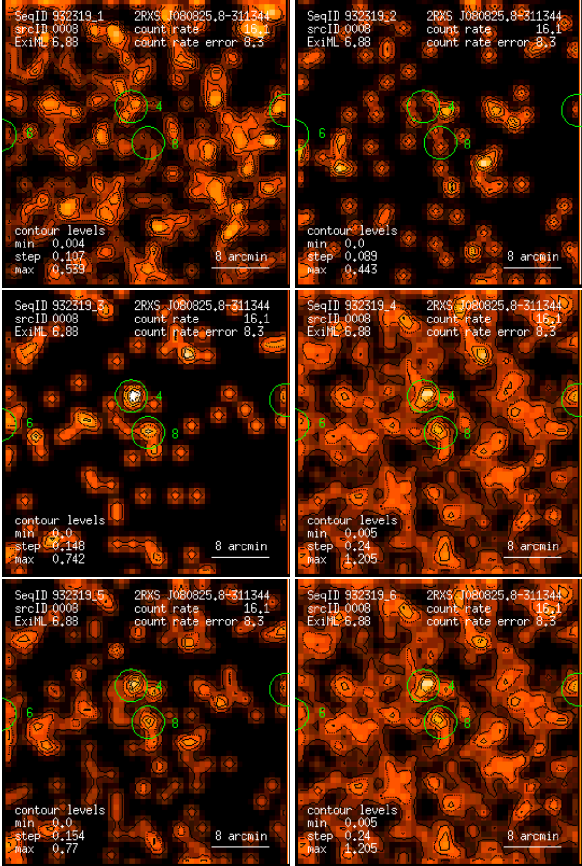
Figure 8: RASS 932319: detection 0008: band rate images, Gaussian filter: (1) PSPC channels 11 – 41, (2) 52 – 90, (3) 91 – 201, (4) 11 – 235, (5) 52 – 201, (6) 11 – 201. Broad band rates in counts/ks. Band rate contour levels in counts/ks/arcmin 2 .
