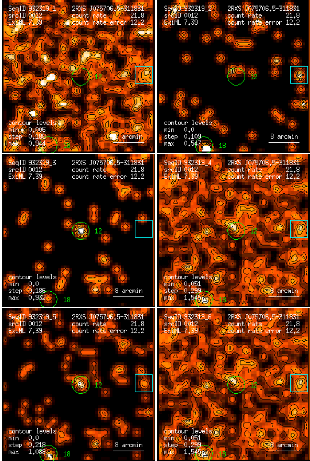
Figure 12: RASS 932319: detection 0012: band rate images, Gaussian filter: (1) PSPC channels 11 – 41, (2) 52 – 90, (3) 91 – 201, (4) 11 – 235, (5) 52 – 201, (6) 11 – 201. Broad band rates in counts/ks. Band rate contour levels in counts/ks/arcmin 2 .
