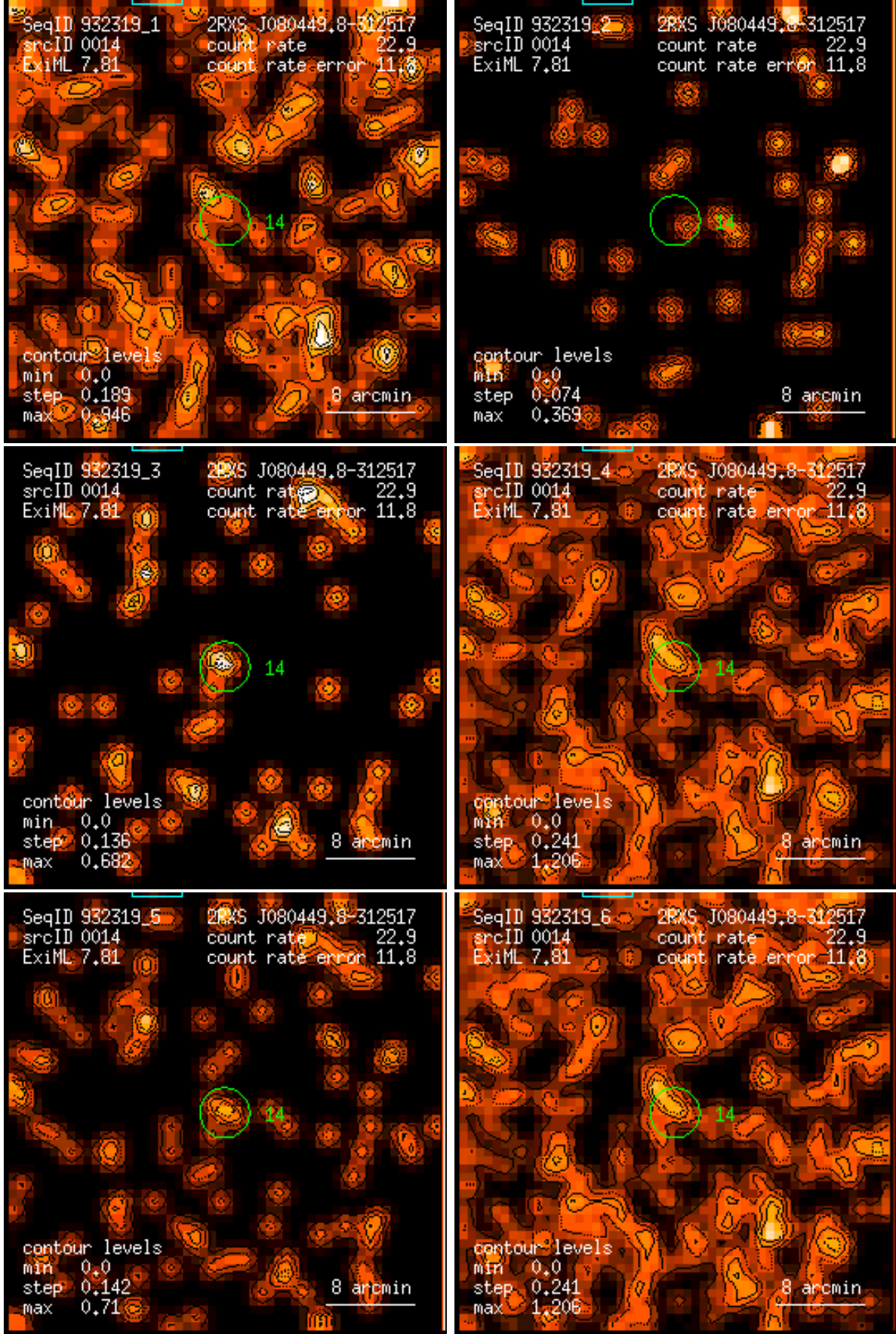
Figure 14: RASS 932319: detection 0014: band rate images, Gaussian filter: (1) PSPC channels 11 – 41, (2) 52 – 90, (3) 91 – 201, (4) 11 – 235, (5) 52 – 201, (6) 11 – 201. Broad band rates in counts/ks. Band rate contour levels in counts/ks/arcmin 2 .
