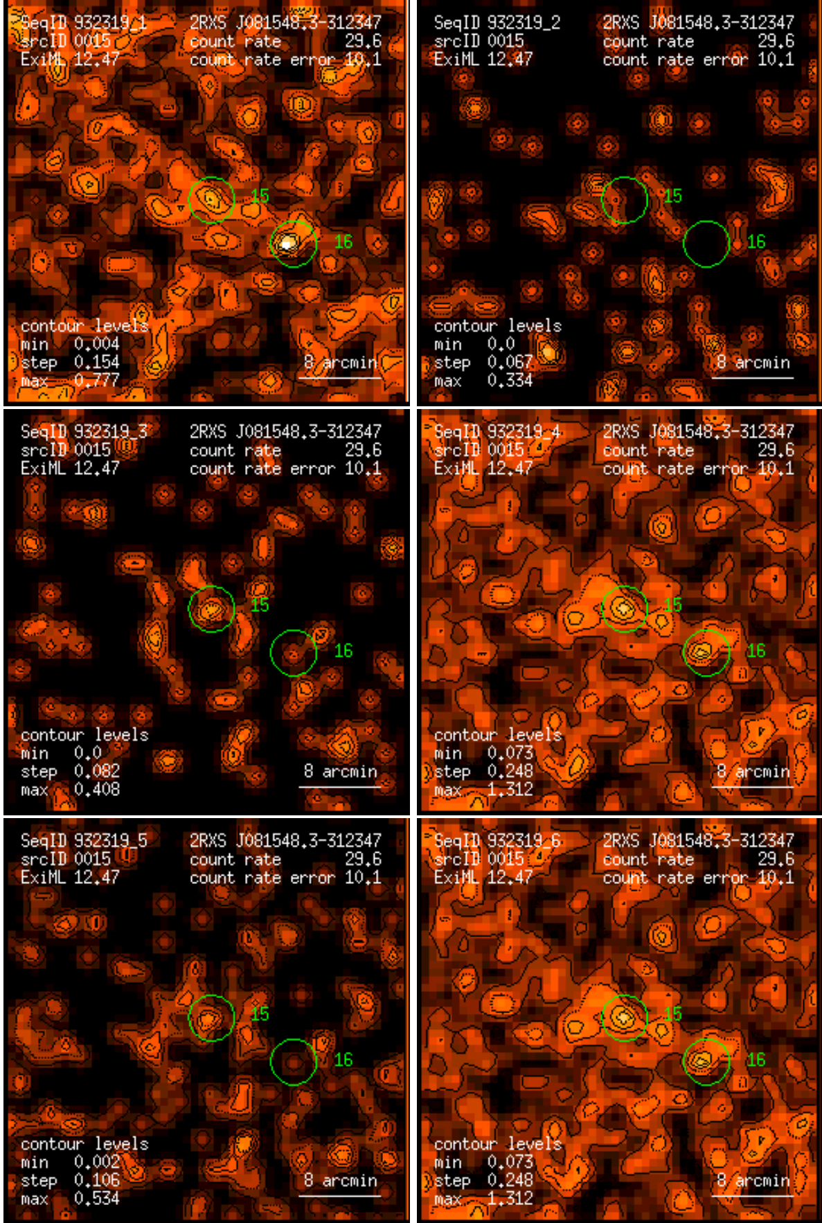
Figure 15: RASS 932319: detection 0015: band rate images, Gaussian filter: (1) PSPC channels 11 – 41, (2) 52 – 90, (3) 91 – 201, (4) 11 – 235, (5) 52 – 201, (6) 11 – 201. Broad band rates in counts/ks. Band rate contour levels in counts/ks/arcmin 2 .
