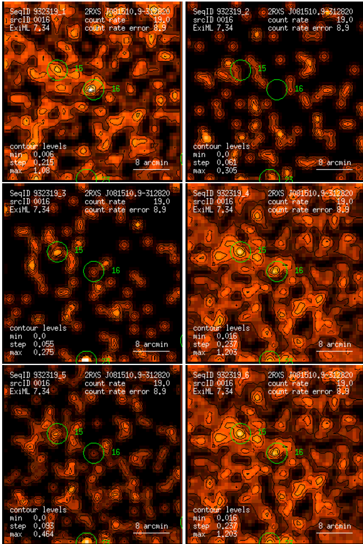
Figure 16: RASS 932319: detection 0016: band rate images, Gaussian filter: (1) PSPC channels 11 – 41, (2) 52 – 90, (3) 91 – 201, (4) 11 – 235, (5) 52 – 201, (6) 11 – 201. Broad band rates in counts/ks. Band rate contour levels in counts/ks/arcmin 2 .
