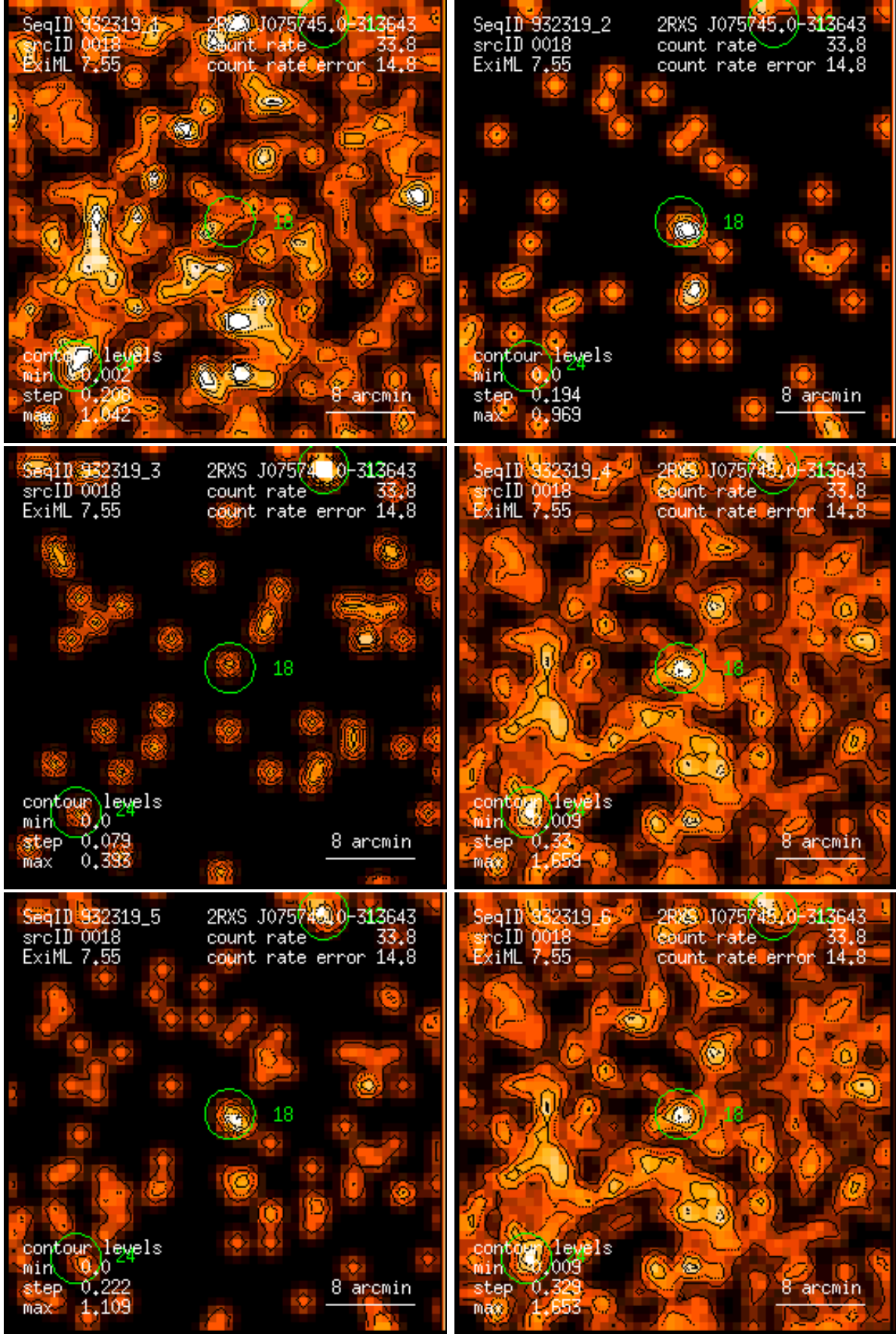
Figure 18: RASS 932319: detection 0018: band rate images, Gaussian filter: (1) PSPC channels 11 – 41, (2) 52 – 90, (3) 91 – 201, (4) 11 – 235, (5) 52 – 201, (6) 11 – 201. Broad band rates in counts/ks. Band rate contour levels in counts/ks/arcmin 2 .
