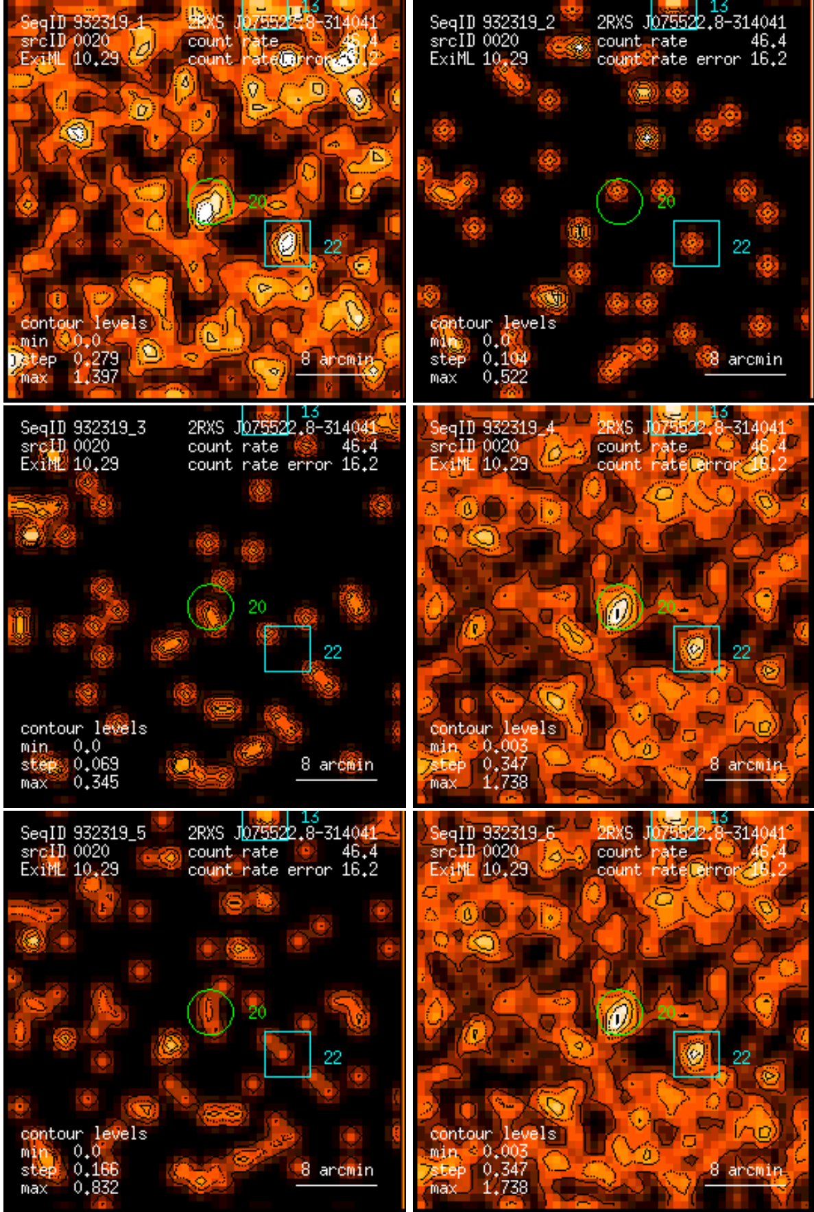
Figure 20: RASS 932319: detection 0020: band rate images, Gaussian filter: (1) PSPC channels 11 – 41, (2) 52 – 90, (3) 91 – 201, (4) 11 – 235, (5) 52 – 201, (6) 11 – 201. Broad band rates in counts/ks. Band rate contour levels in counts/ks/arcmin 2 .
