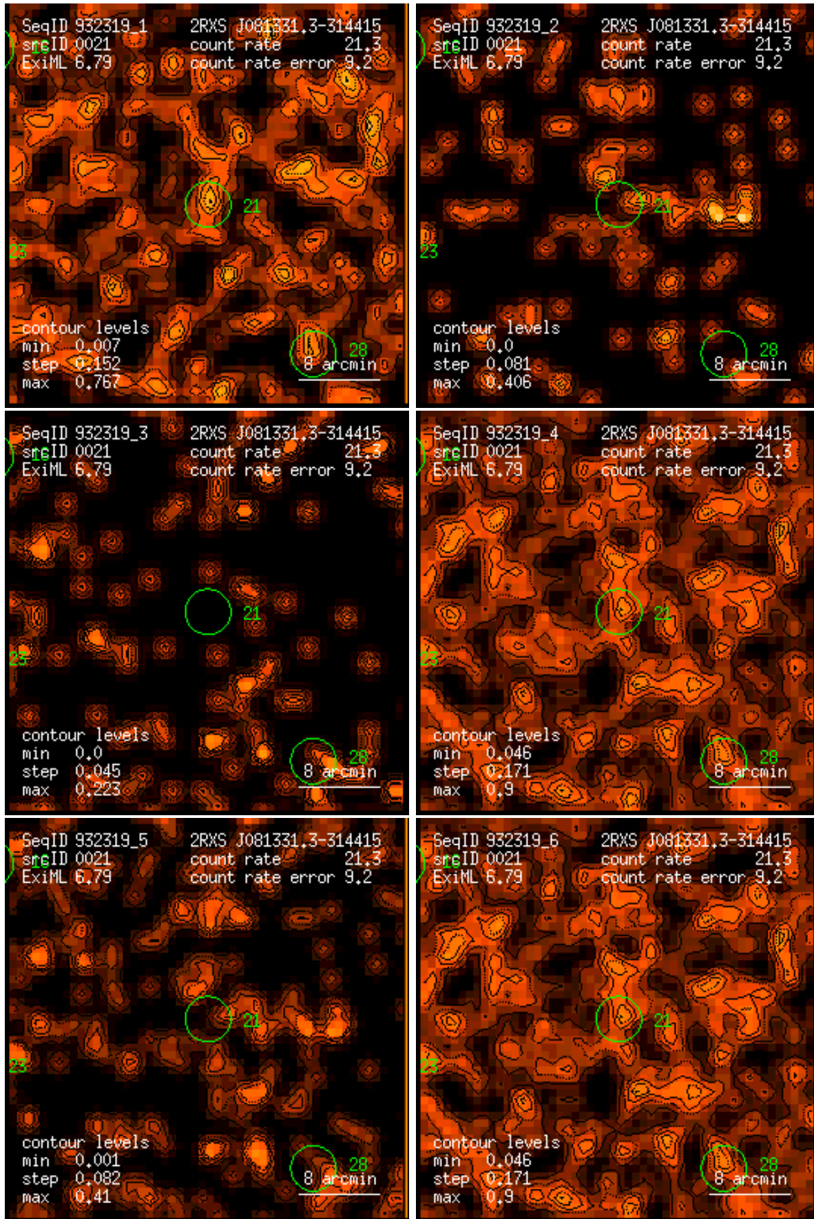
Figure 21: RASS 932319: detection 0021: band rate images, Gaussian filter: (1) PSPC channels 11 – 41, (2) 52 – 90, (3) 91 – 201, (4) 11 – 235, (5) 52 – 201, (6) 11 – 201. Broad band rates in counts/ks. Band rate contour levels in counts/ks/arcmin 2 .
