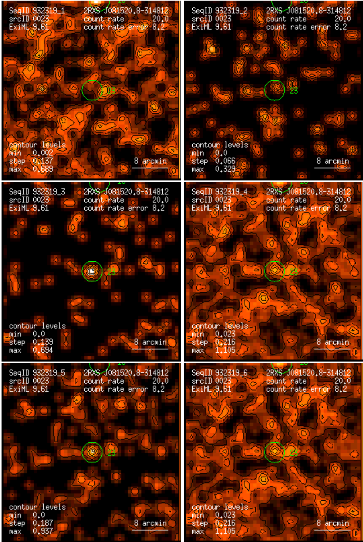
Figure 23: RASS 932319: detection 0023: band rate images, Gaussian filter: (1) PSPC channels 11 – 41, (2) 52 – 90, (3) 91 – 201, (4) 11 – 235, (5) 52 – 201, (6) 11 – 201. Broad band rates in counts/ks. Band rate contour levels in counts/ks/arcmin 2 .
