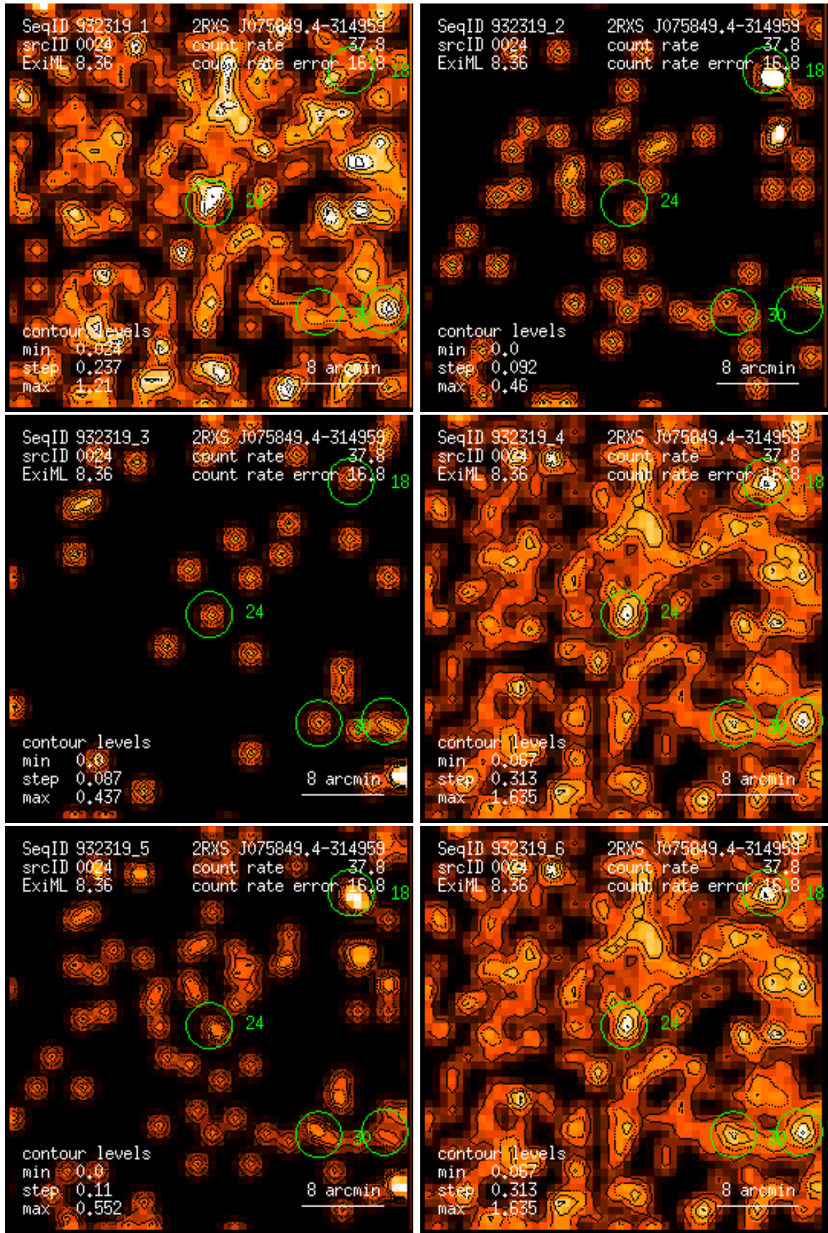
Figure 24: RASS 932319: detection 0024: band rate images, Gaussian filter: (1) PSPC channels 11 – 41, (2) 52 – 90, (3) 91 – 201, (4) 11 – 235, (5) 52 – 201, (6) 11 – 201. Broad band rates in counts/ks. Band rate contour levels in counts/ks/arcmin 2 .
