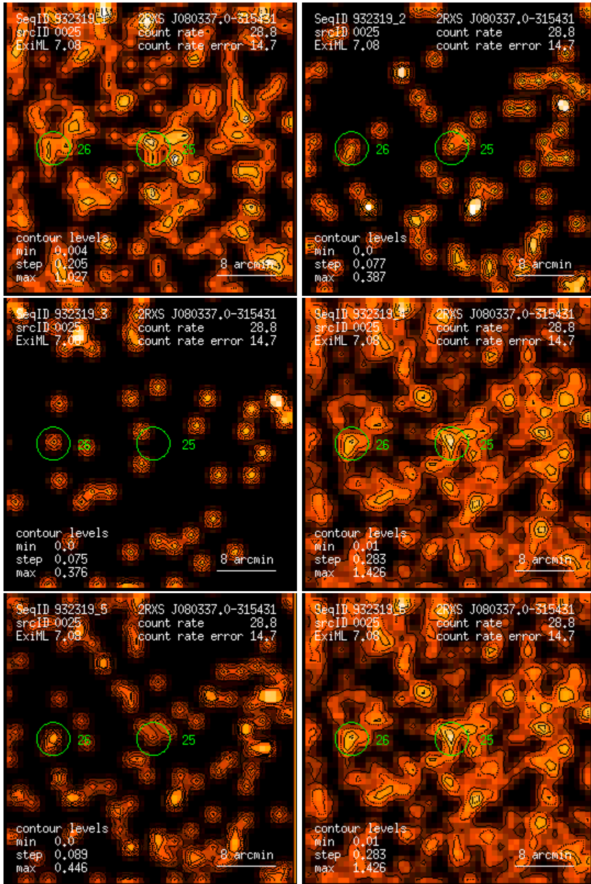
Figure 25: RASS 932319: detection 0025: band rate images, Gaussian filter: (1) PSPC channels 11 – 41, (2) 52 – 90, (3) 91 – 201, (4) 11 – 235, (5) 52 – 201, (6) 11 – 201. Broad band rates in counts/ks. Band rate contour levels in counts/ks/arcmin 2 .
