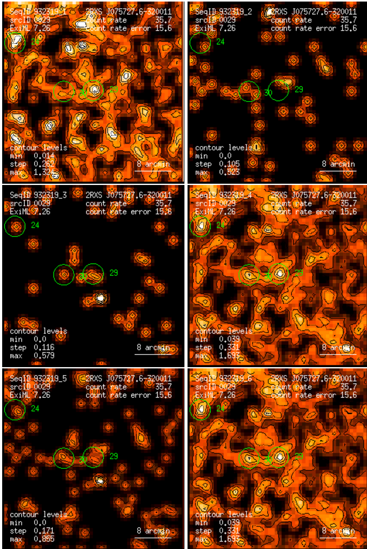
Figure 29: RASS 932319: detection 0029: band rate images, Gaussian filter: (1) PSPC channels 11 – 41, (2) 52 – 90, (3) 91 – 201, (4) 11 – 235, (5) 52 – 201, (6) 11 – 201. Broad band rates in counts/ks. Band rate contour levels in counts/ks/arcmin 2 .
