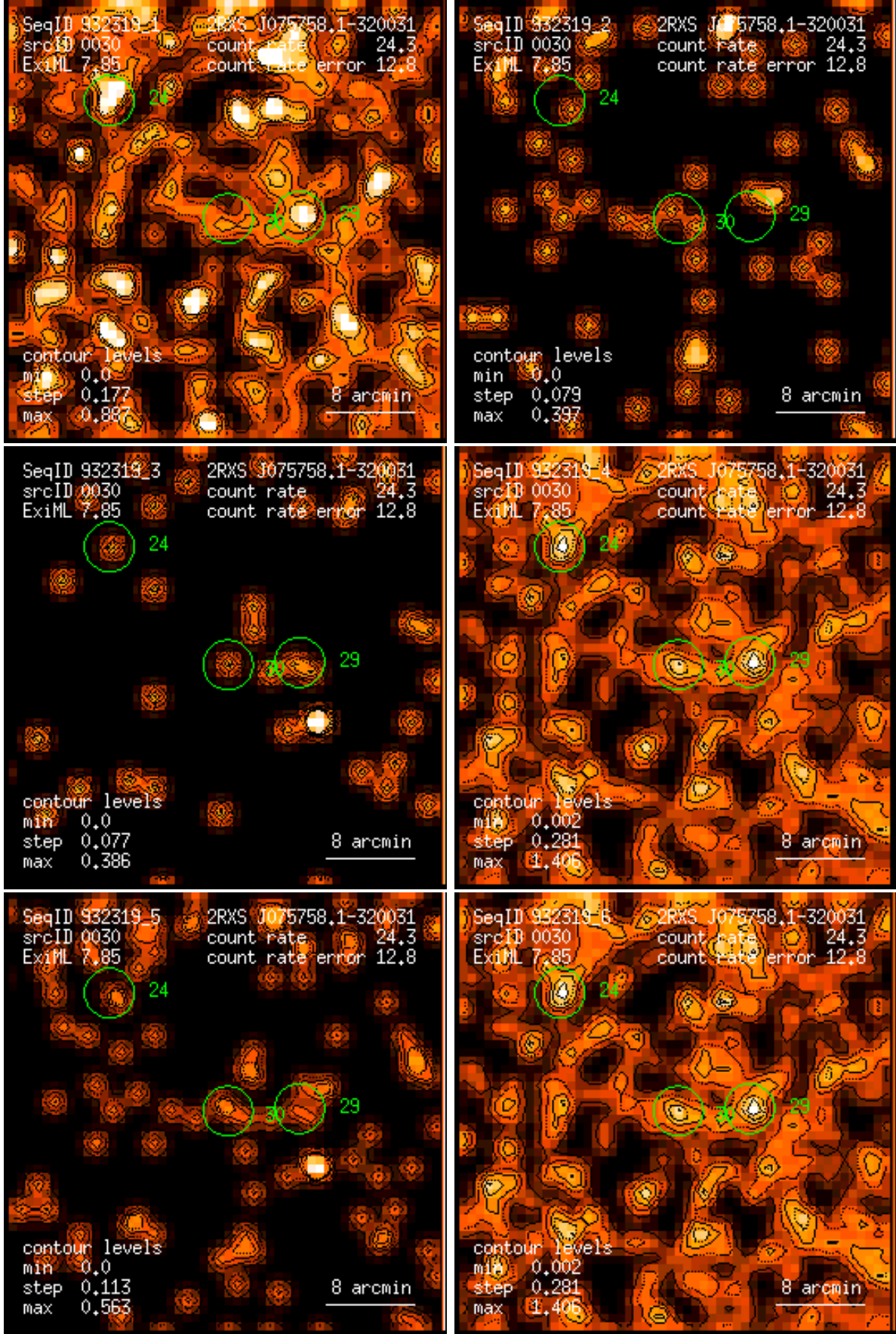
Figure 30: RASS 932319: detection 0030: band rate images, Gaussian filter: (1) PSPC channels 11 – 41, (2) 52 – 90, (3) 91 – 201, (4) 11 – 235, (5) 52 – 201, (6) 11 – 201. Broad band rates in counts/ks. Band rate contour levels in counts/ks/arcmin 2 .
