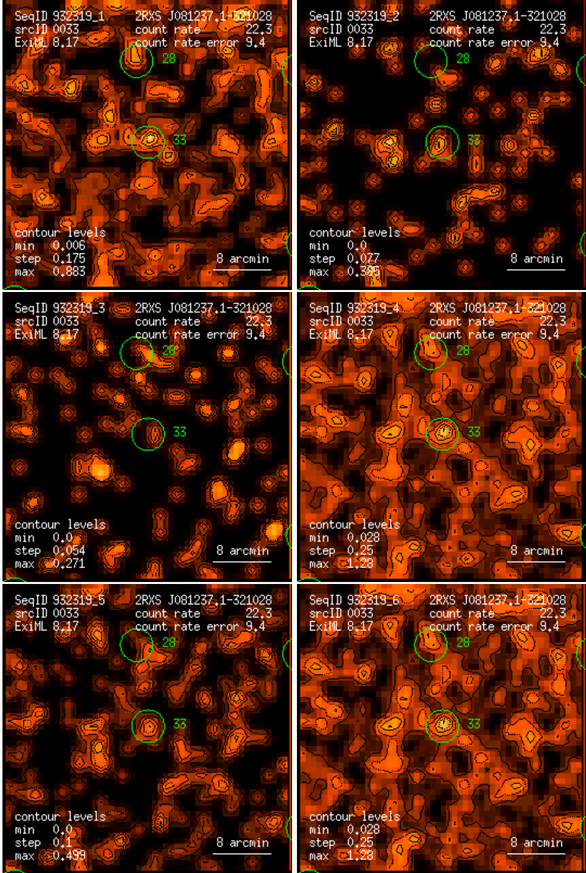
Figure 33: RASS 932319: detection 0033: band rate images, Gaussian filter: (1) PSPC channels 11 – 41, (2) 52 – 90, (3) 91 – 201, (4) 11 – 235, (5) 52 – 201, (6) 11 – 201. Broad band rates in counts/ks. Band rate contour levels in counts/ks/arcmin 2 .
