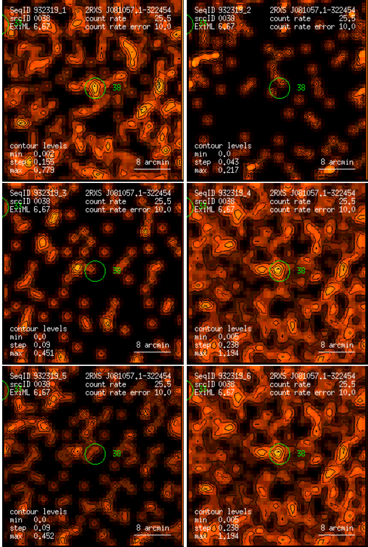
Figure 38: RASS 932319: detection 0038: band rate images, Gaussian filter: (1) PSPC channels 11 – 41, (2) 52 – 90, (3) 91 – 201, (4) 11 – 235, (5) 52 – 201, (6) 11 – 201. Broad band rates in counts/ks. Band rate contour levels in counts/ks/arcmin 2 .
