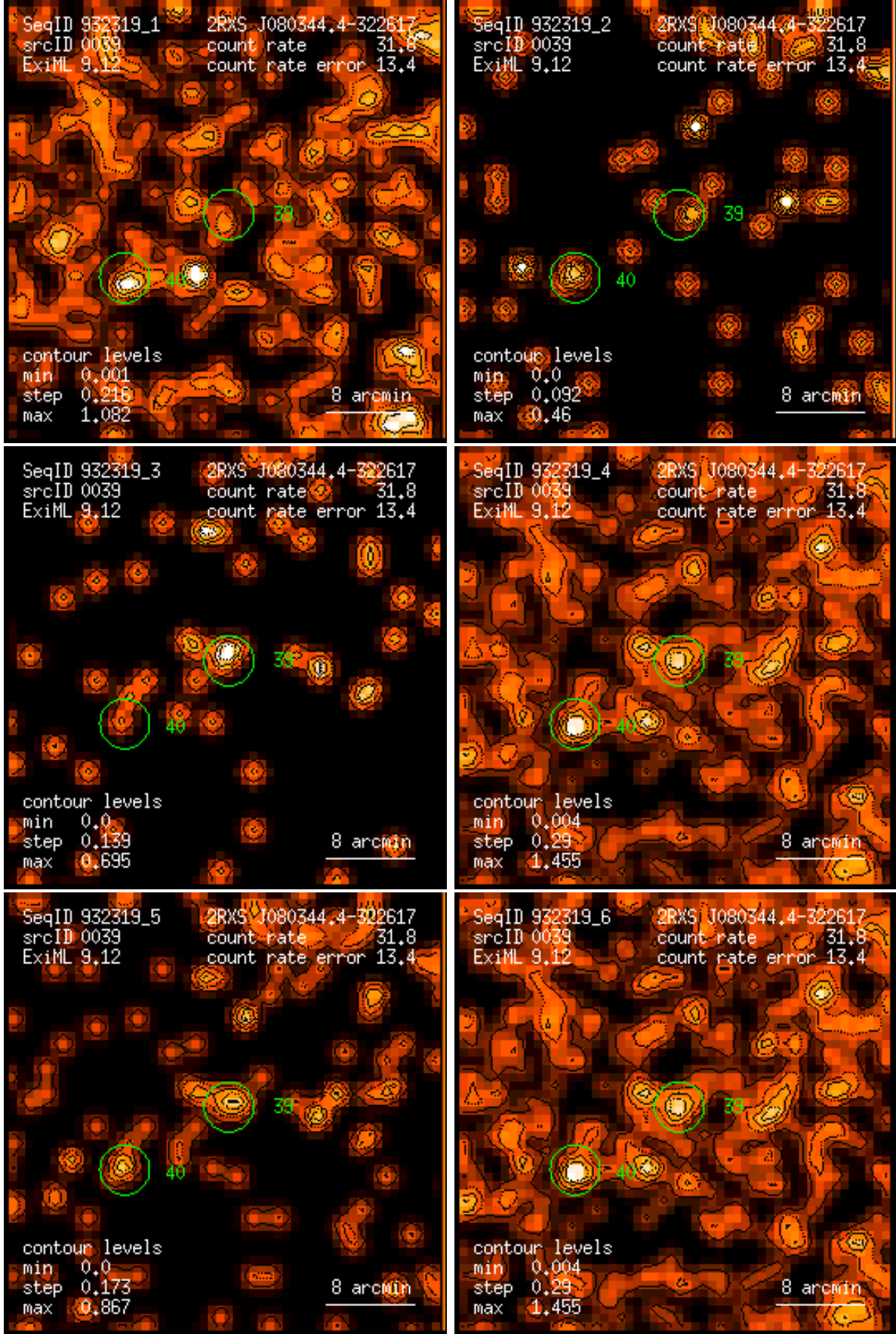
Figure 39: RASS 932319: detection 0039: band rate images, Gaussian filter: (1) PSPC channels 11 – 41, (2) 52 – 90, (3) 91 – 201, (4) 11 – 235, (5) 52 – 201, (6) 11 – 201. Broad band rates in counts/ks. Band rate contour levels in counts/ks/arcmin 2 .
