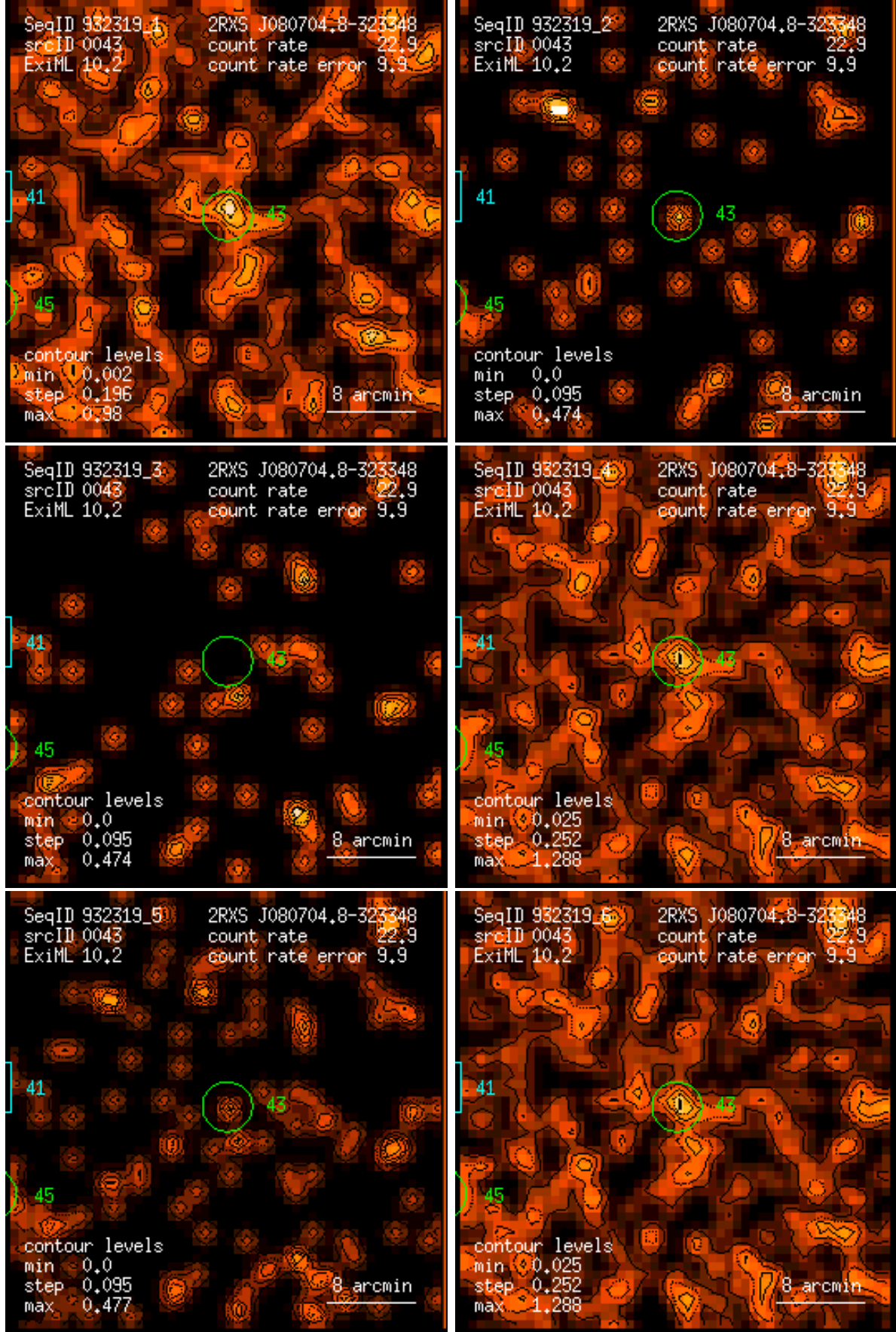
Figure 43: RASS 932319: detection 0043: band rate images, Gaussian filter: (1) PSPC channels 11 – 41, (2) 52 – 90, (3) 91 – 201, (4) 11 – 235, (5) 52 – 201, (6) 11 – 201. Broad band rates in counts/ks. Band rate contour levels in counts/ks/arcmin 2 .
