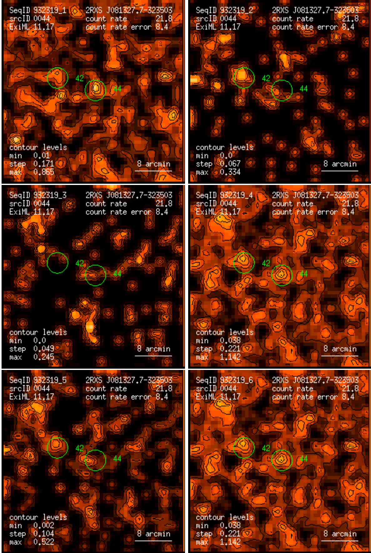
Figure 44: RASS 932319: detection 0044: band rate images, Gaussian filter: (1) PSPC channels 11 – 41, (2) 52 – 90, (3) 91 – 201, (4) 11 – 235, (5) 52 – 201, (6) 11 – 201. Broad band rates in counts/ks. Band rate contour levels in counts/ks/arcmin 2 .
