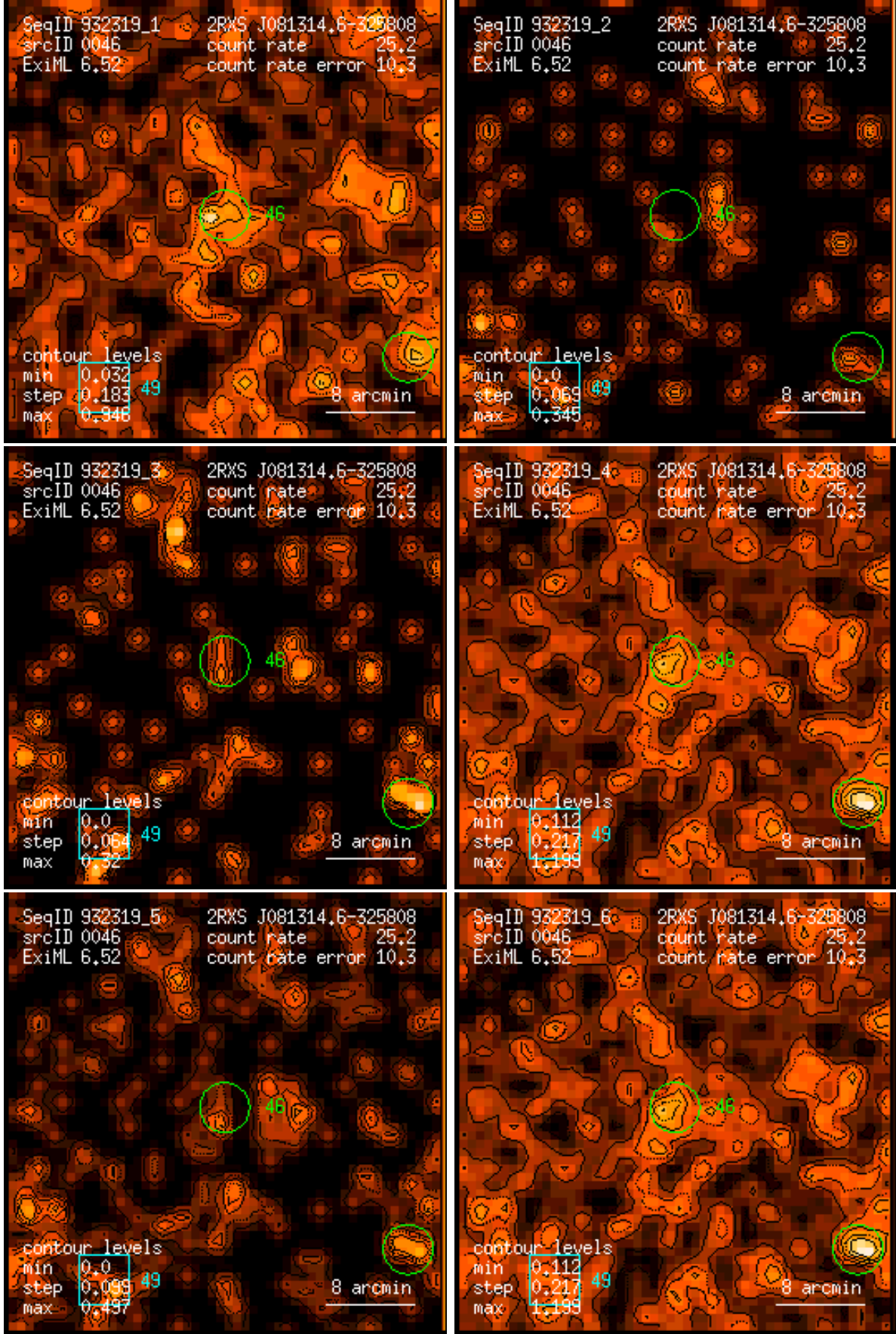
Figure 46: RASS 932319: detection 0046: band rate images, Gaussian filter: (1) PSPC channels 11 – 41, (2) 52 – 90, (3) 91 – 201, (4) 11 – 235, (5) 52 – 201, (6) 11 – 201. Broad band rates in counts/ks. Band rate contour levels in counts/ks/arcmin 2 .
