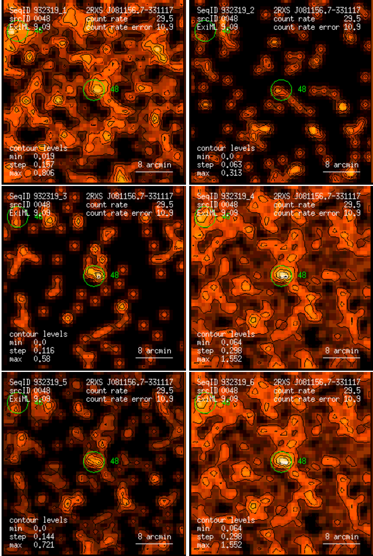
Figure 48: RASS 932319: detection 0048: band rate images, Gaussian filter: (1) PSPC channels 11 – 41, (2) 52 – 90, (3) 91 – 201, (4) 11 – 235, (5) 52 – 201, (6) 11 – 201. Broad band rates in counts/ks. Band rate contour levels in counts/ks/arcmin 2 .
